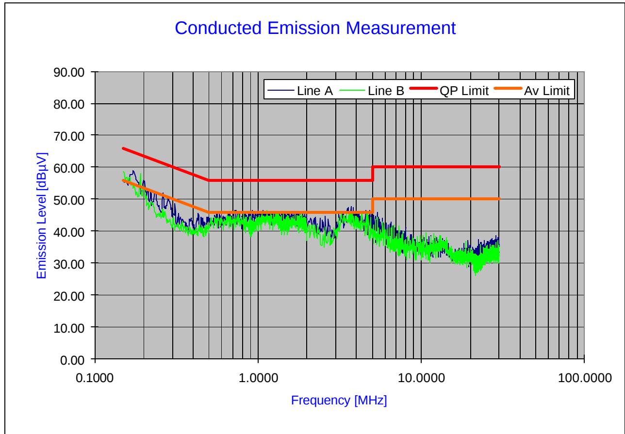
Plot 6-24. Line Conducted Plot with 802.11g
