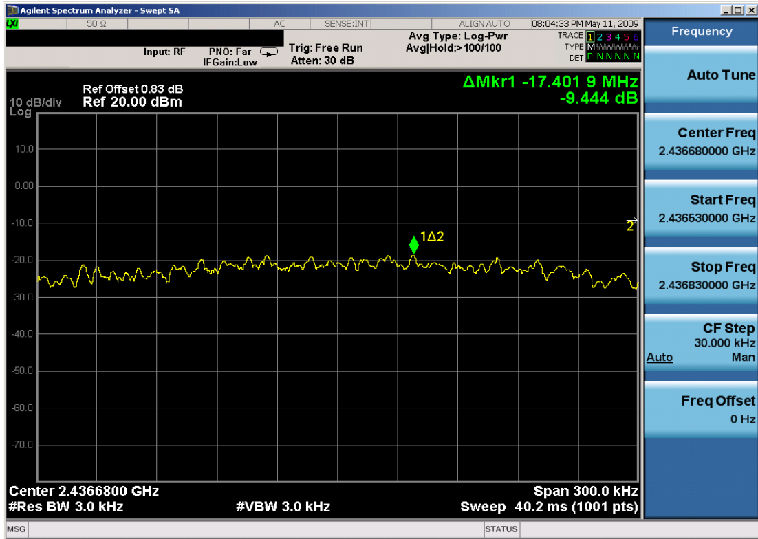
Plot 6-11. Power Spectral Density Plot (802.11g - Ch. 6)
