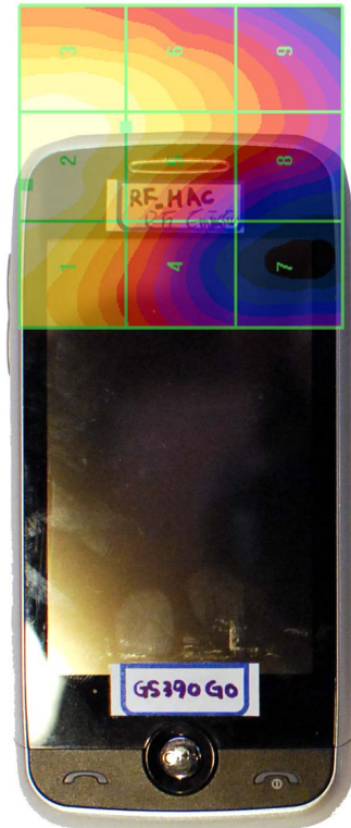
Figure 16-4 E-Field WD Scan overlay
