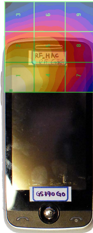
Figure 16-5 H-Field WD Scan overlay
