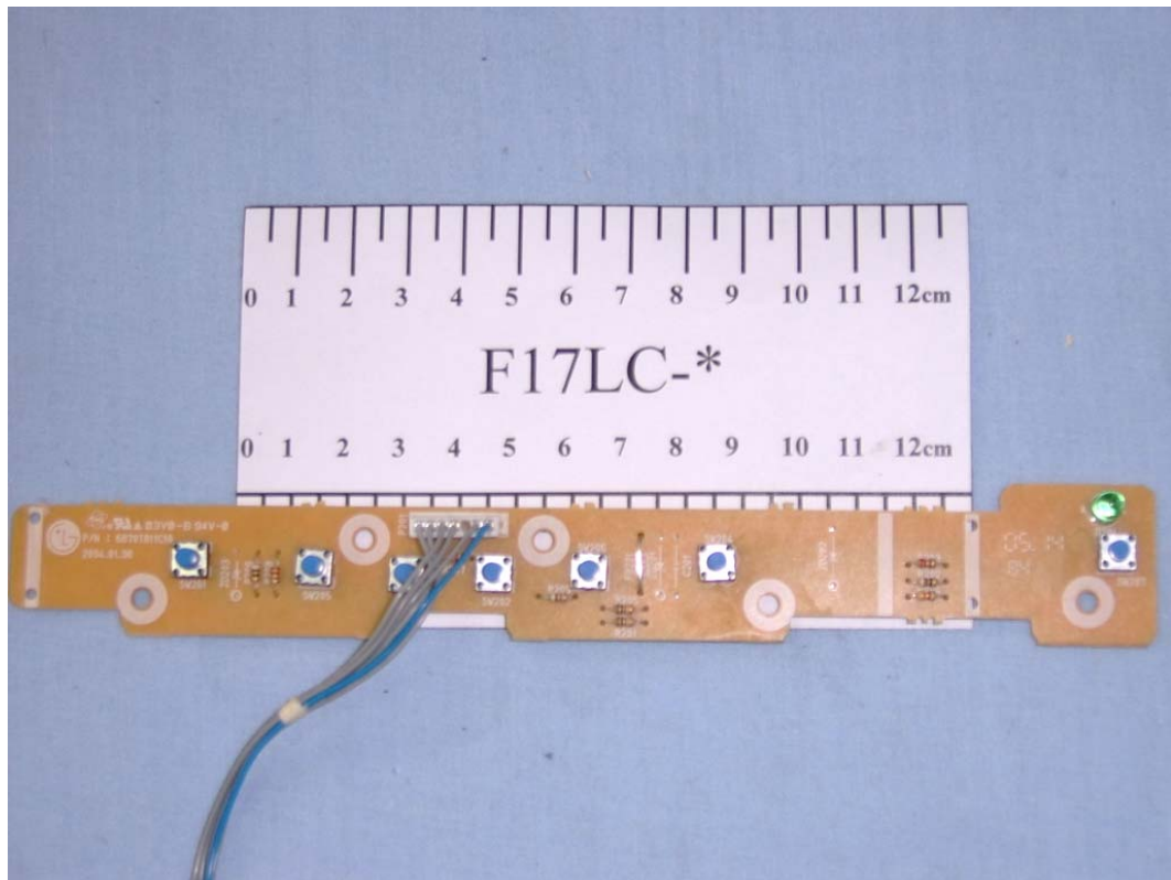
FIGURE 8 COLOR MONITOR (M/N:F17LC-*) CONTROL PANEL BOARD (COMPONENT SIDE)
