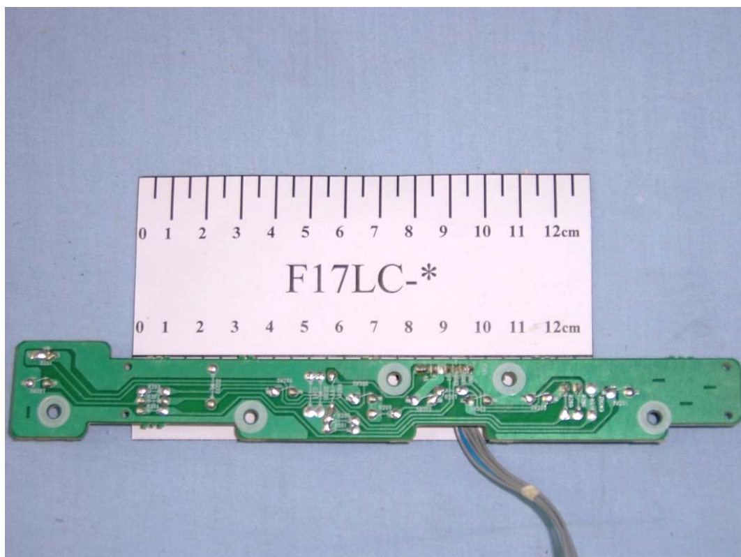
FIGURE 9 COLOR MONITOR (M/N:F17LC-*) CONTROL PANEL BOARD (SOLDERED SIDE)
