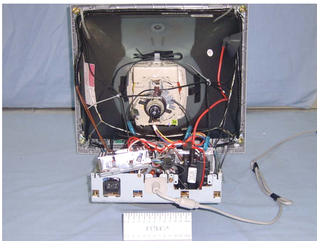
FIGURE 2 COLOR MONITOR (M/N:F17LC-*) COVER REMOVED 2
