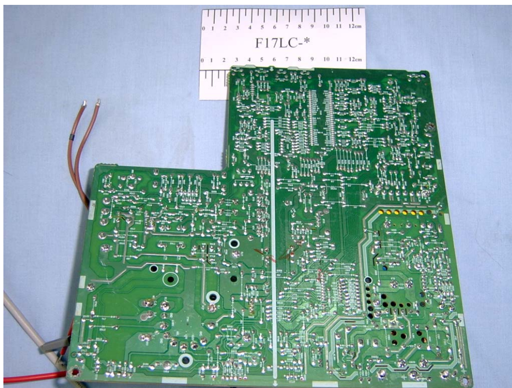
FIGURE 5 COLOR MONITOR (M/N:F17LC-*) MAIN BOARD (SOLDERED SIDE)
