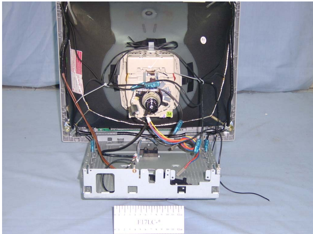
FIGURE 3 COLOR MONITOR (M/N:F17LC-*) CRT TUBE
