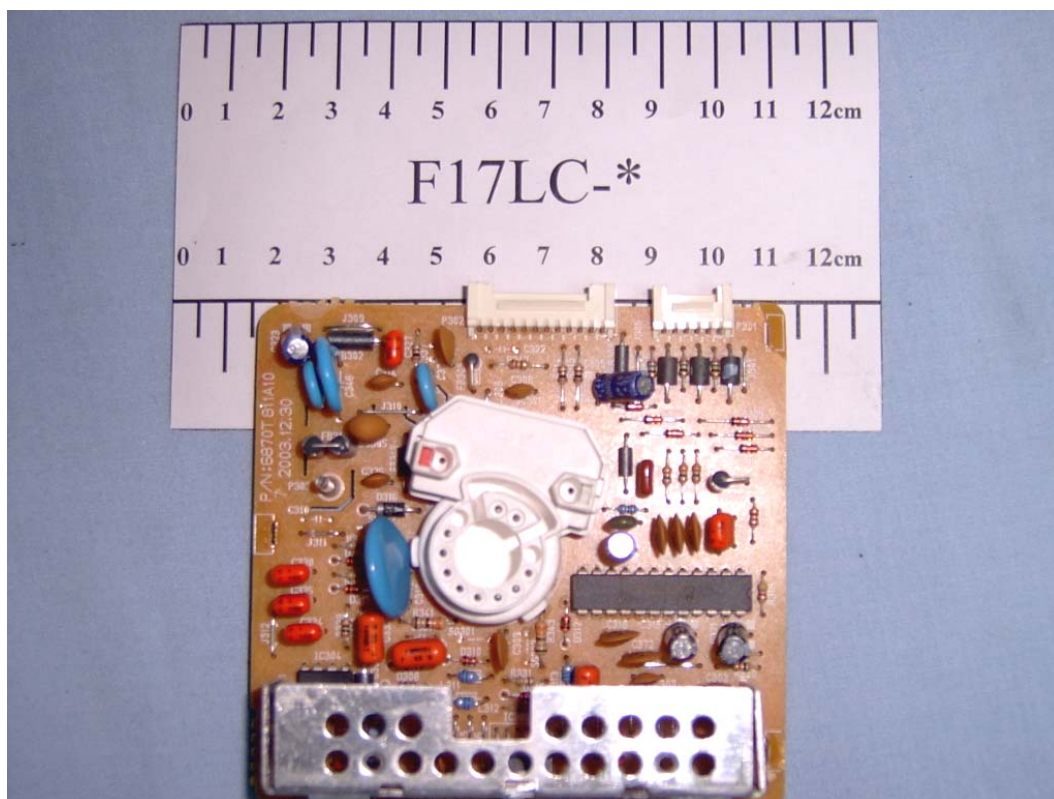
FIGURE 6 COLOR MONITOR (M/N:F17LC-*) CRT BOARD (COMPONENT SIDE)
