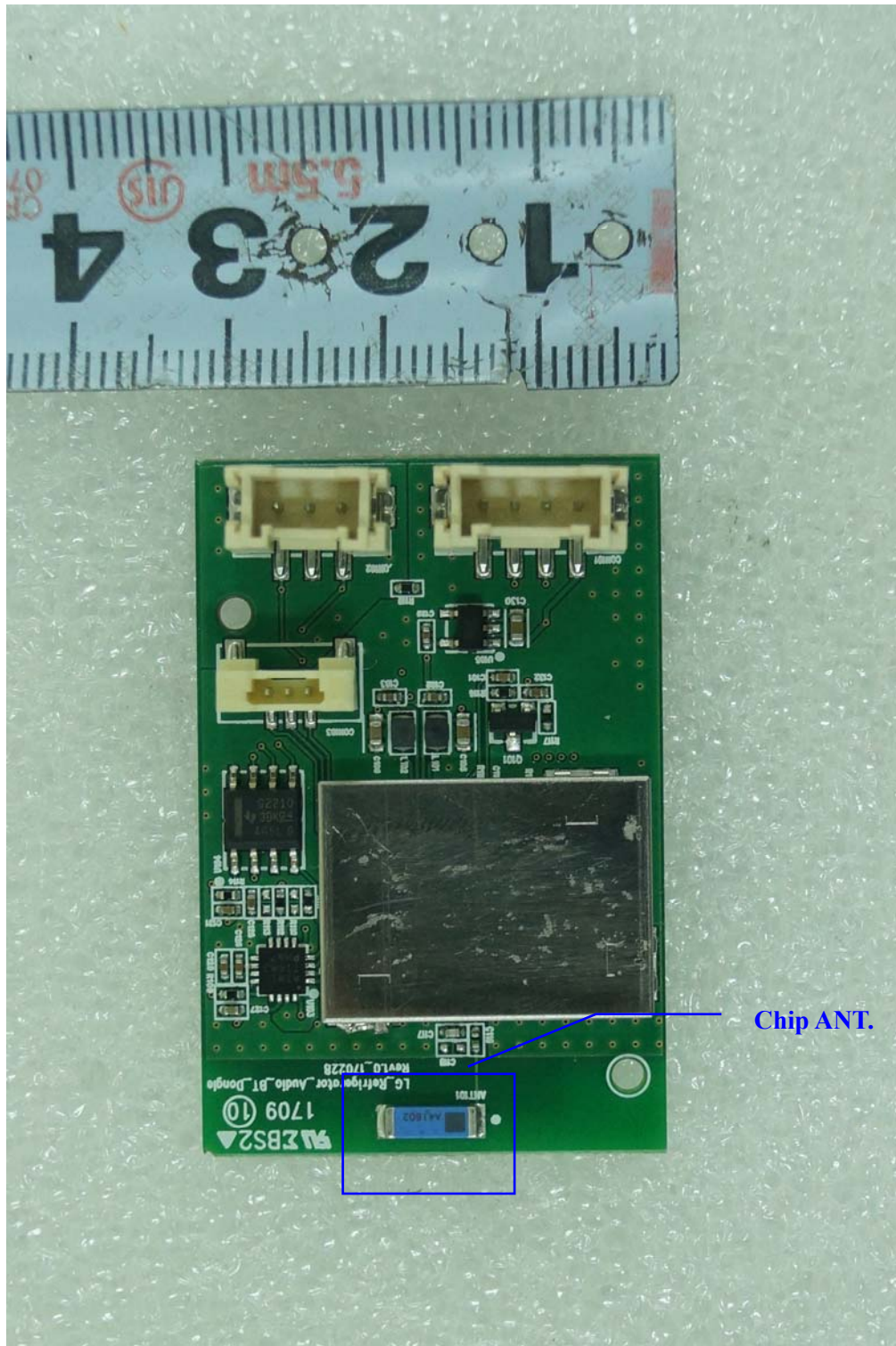
< Top view >
