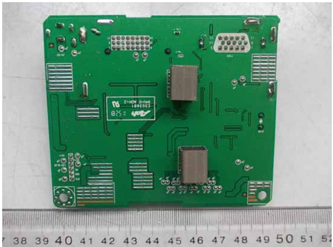
FIGURE 5 LCD MONITOR (M/N: E2442TCA) MAIN BOARD (SOLDERED SIDE)
