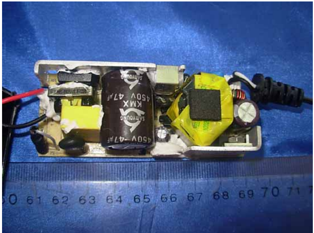
FIGURE 14 LCD MONITOR (M/N: E1948SX) ADAPTOR#2 (MAIN BOARD – COMPONENT SIDE)
