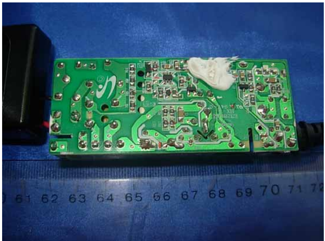
FIGURE 15 LCD MONITOR (M/N: E1948SX) ADAPTOR#2 (MAIN BOARD – SOLDERED SIDE)
