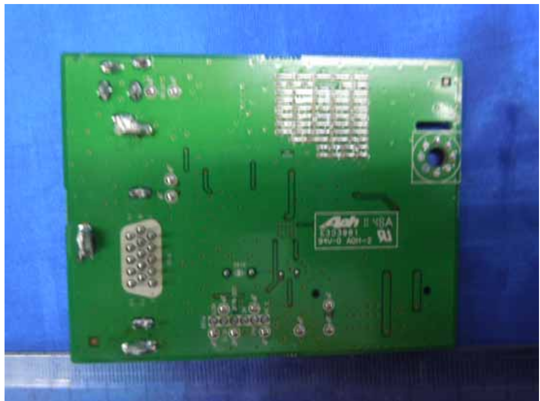
FIGURE 4 LCD MONITOR (M/N: E1642CA) MAIN BOARD (SOLDERED SIDE)
