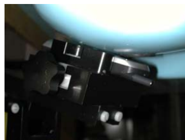
Figure 16. Left Head SAR Test Setup -- Check / Touch Position --
