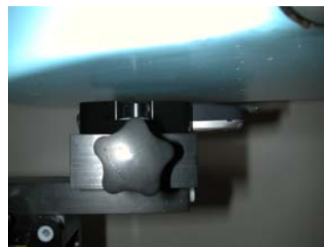
Figure 22. Body SAR Test Setup
