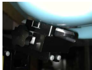
Figure 20. Left Head SAR Test Setup -- Check / Touch Position --
