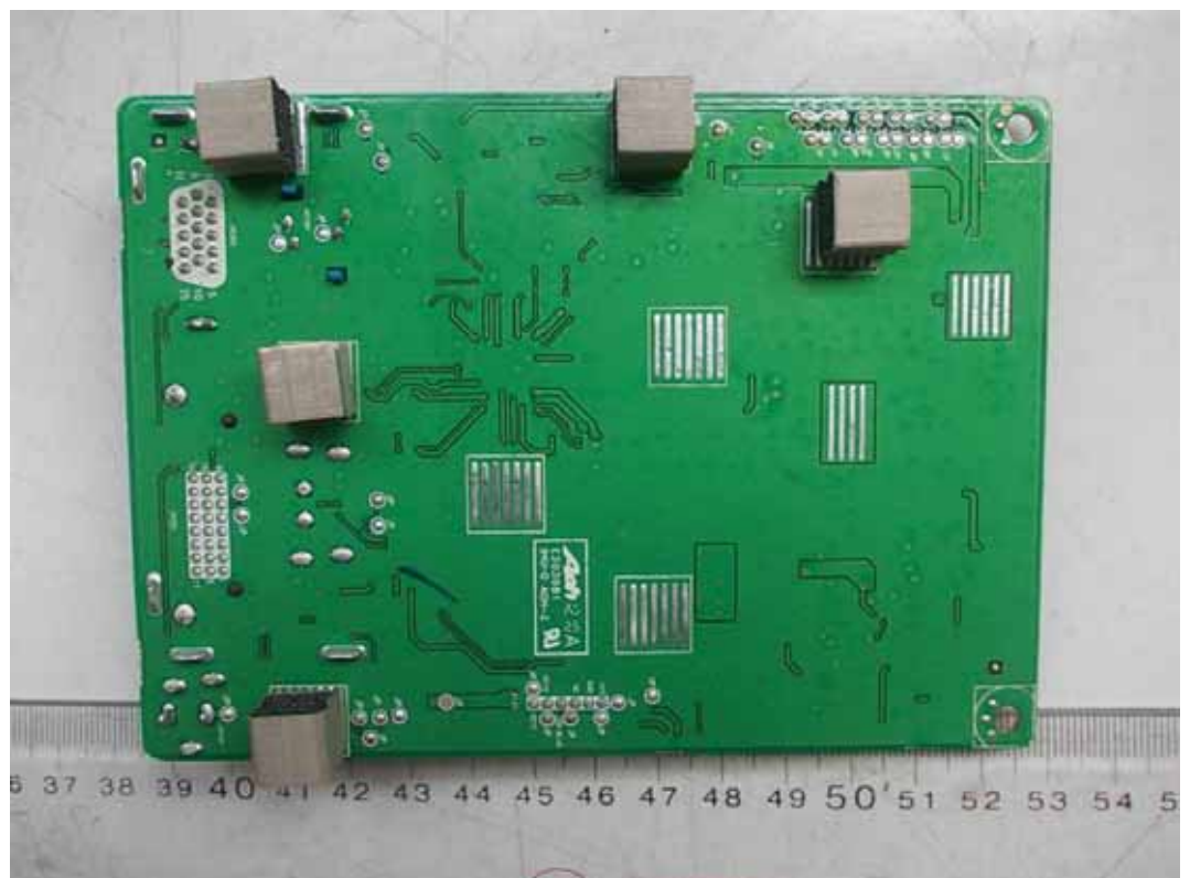
FIGURE 4 LCD MONITOR (M/N: D2343PB) MAIN BOARD (SOLDERED SIDE)
