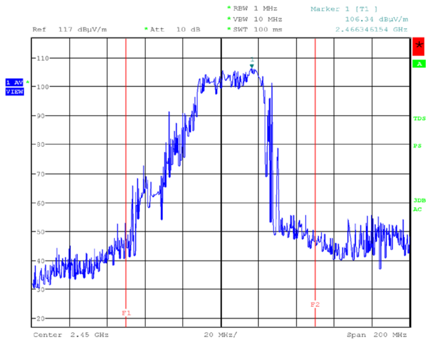
< Fig 10. Frequency Measurements_Voltage (Minimum Frequency Observed: 2.466 GHz) >
