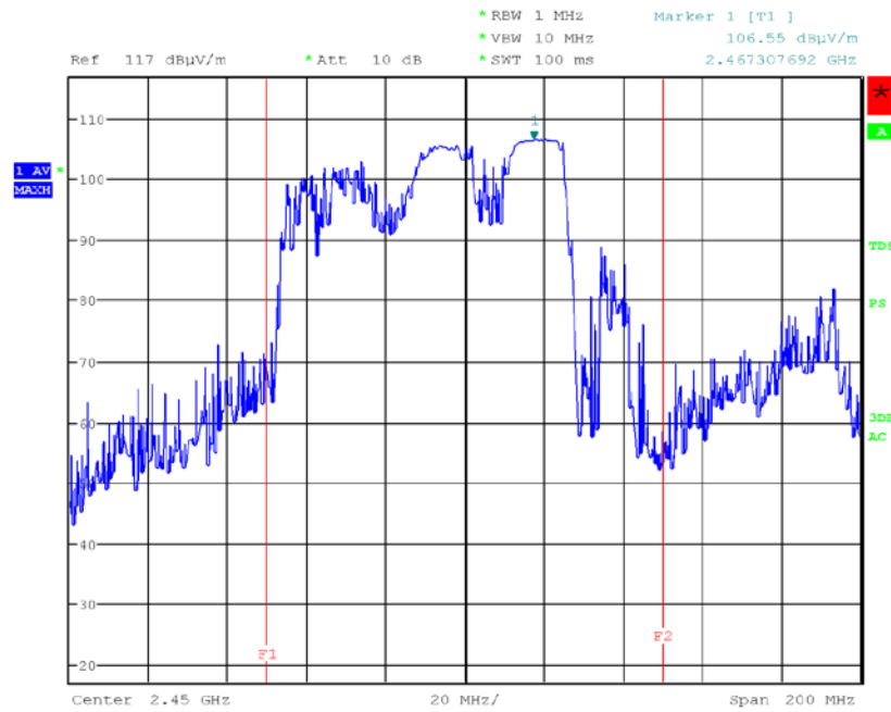
< Fig 7. Frequency Measurements_Load (Maximum Frequency Observed: 2.467 GHz) >
