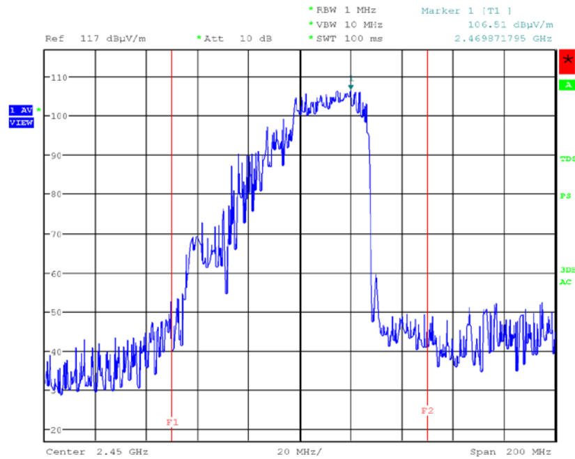
< Fig 9. Frequency Measurements_Voltage (Maximum Frequency Observed: 2.469 GHz) >
