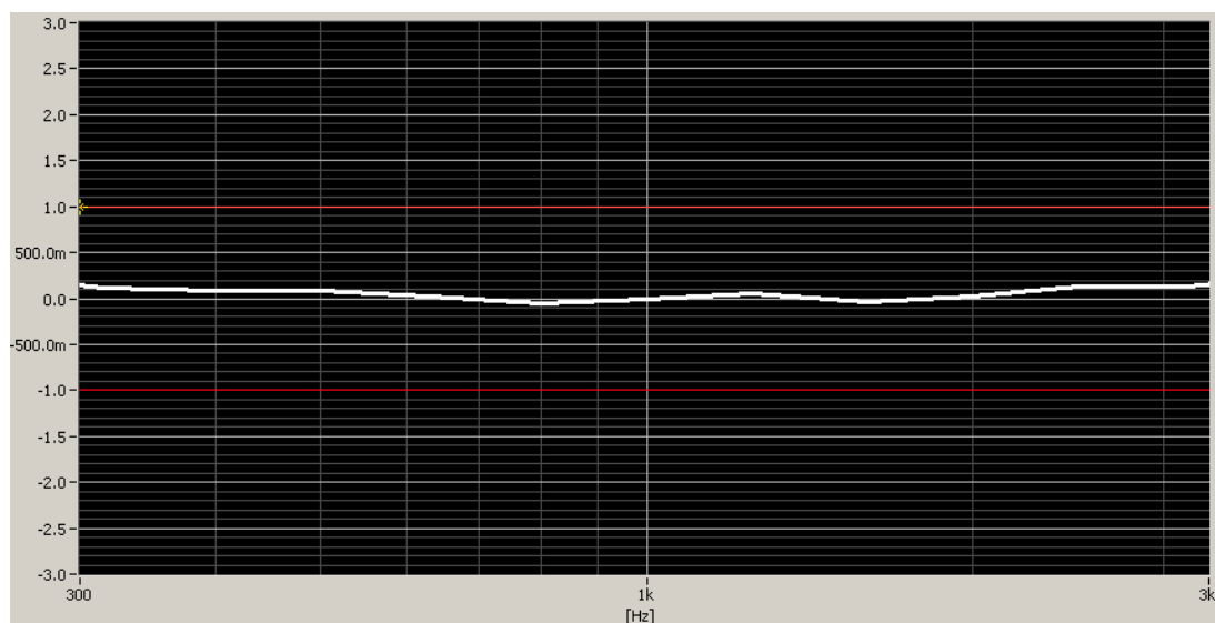
Figure 7-3 Helmholtz Coil Validation for Frequency Response
