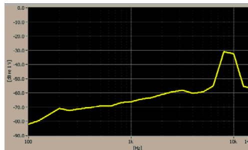
Figure 7-2 Worst-case ABM2 Plot for WD
