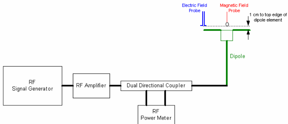
Figure 17 System Check Setup
