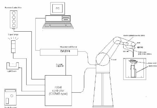
Figure 7 SPEAG Robotic System Diagram
