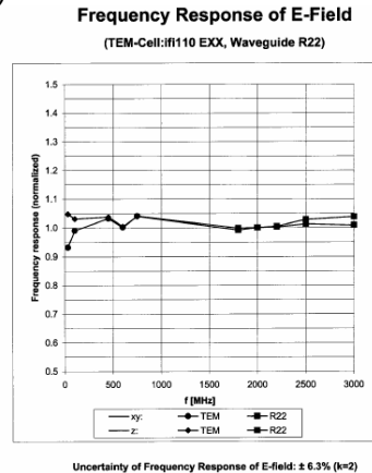
Figure 4 E-Field Probe Frequency Response
