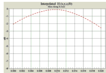
Figure 16 2-D Interpolated points from scan along transverse axis
