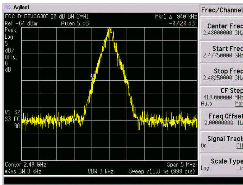
Plot A-3. 20dB Bandwidth Plot – Ch. 78
