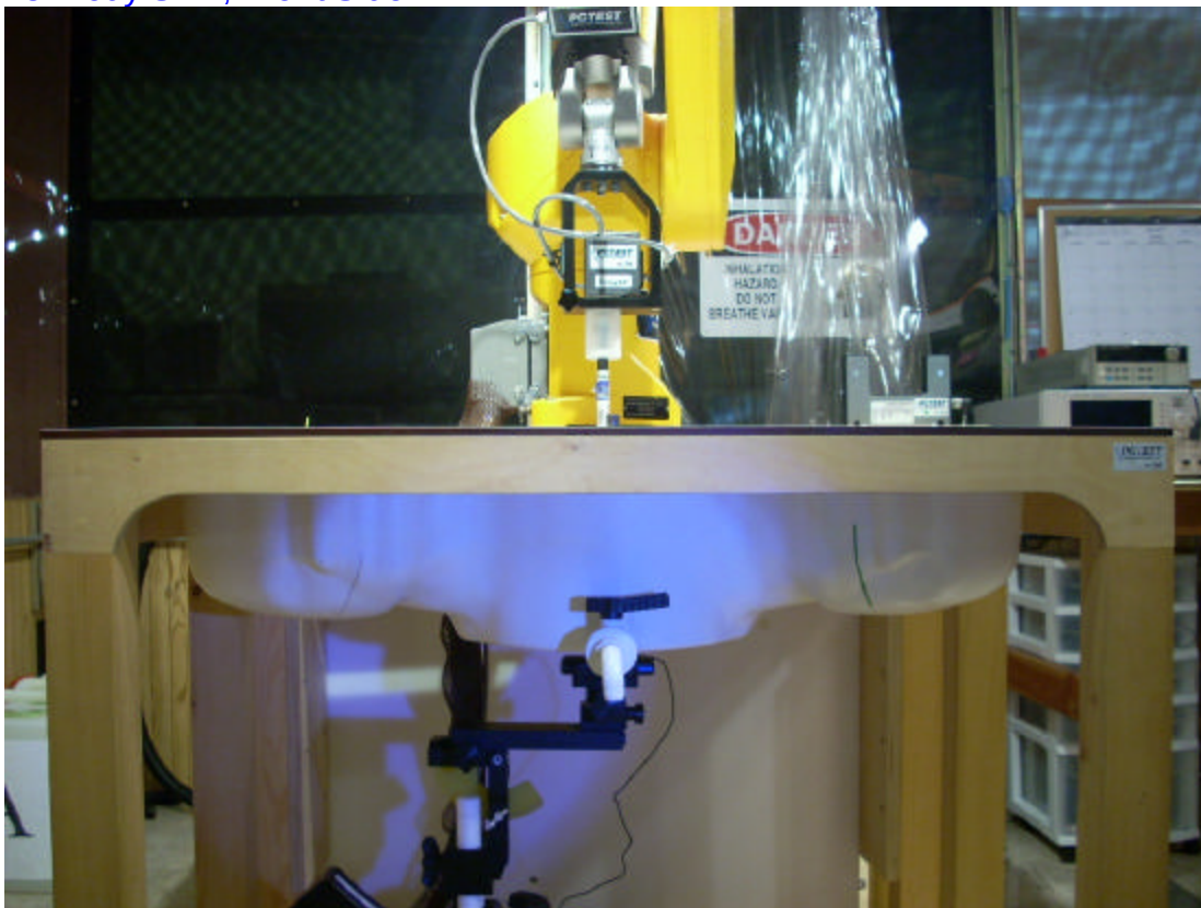
14. Body SAR, Front Side with 20mm Space
