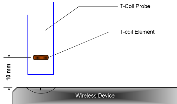
Figure 5-11 Measurement Distance
