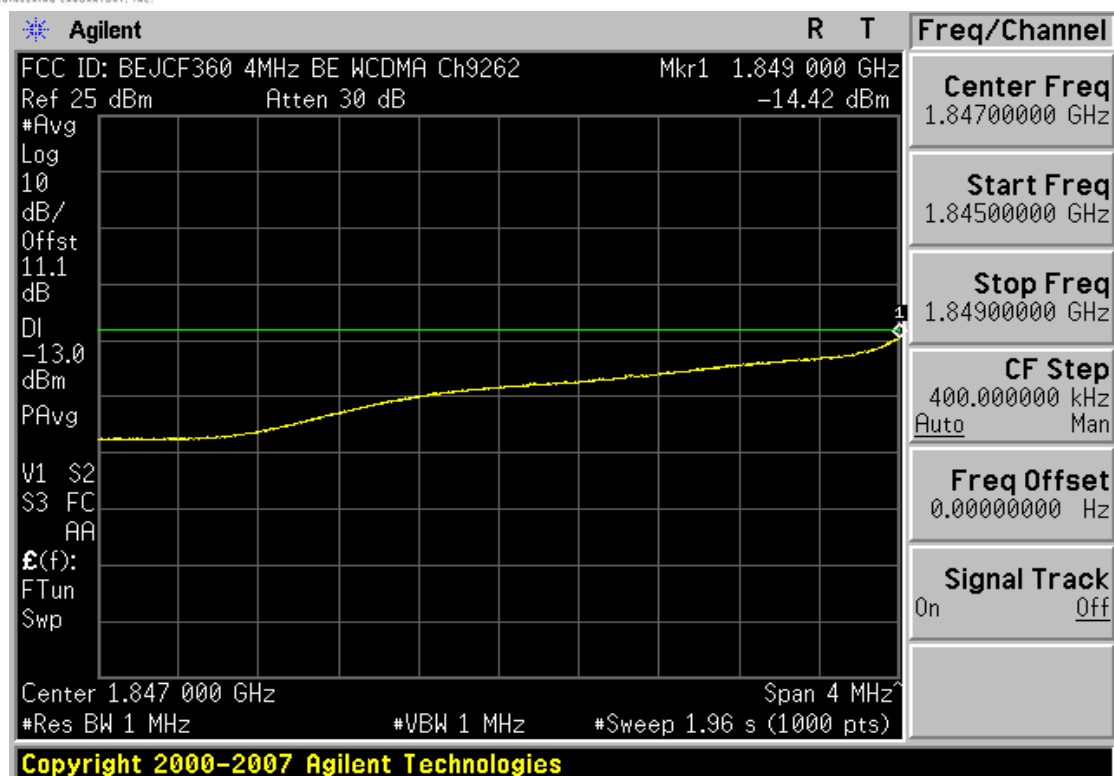
Plot 7-36. 4MHz Span Plot (PCS WCDMA Mode – Ch. 9262)
