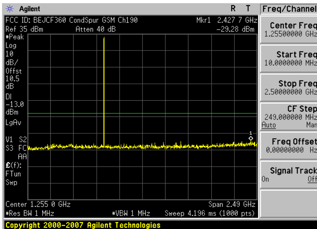
Plot 7-4. Conducted Spurios (Cellular GSM Mode – Ch. 190)
