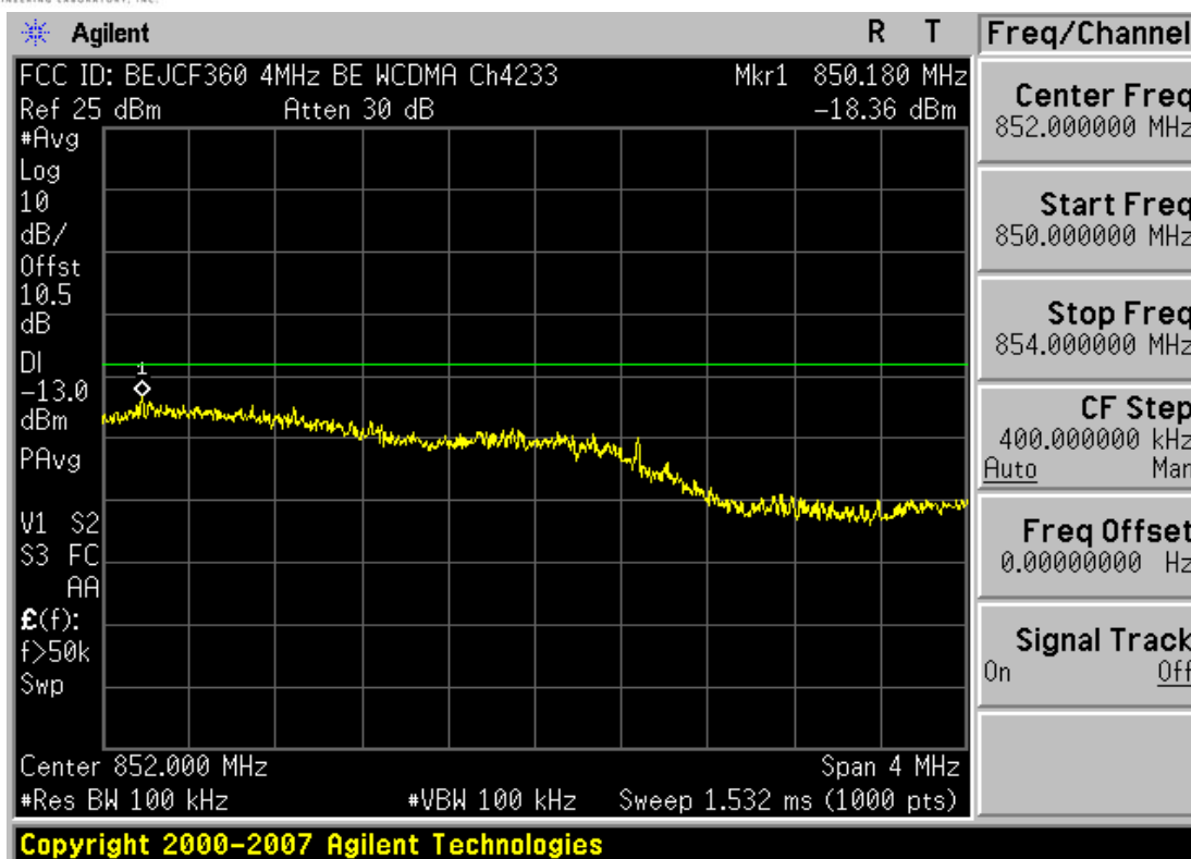
Plot 7-32. 4MHz Span Plot (Cellular WCDMA Mode – Ch. 4233)
