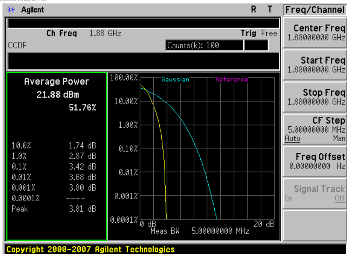
Plot 7-40. Peak-Average Ratio Plot (PCS WCDMA Mode - Ch. 9400)
