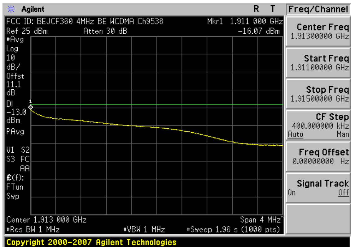
Plot 7-44. 4MHz Span Plot (PCS WCDMA Mode – Ch. 9538)
