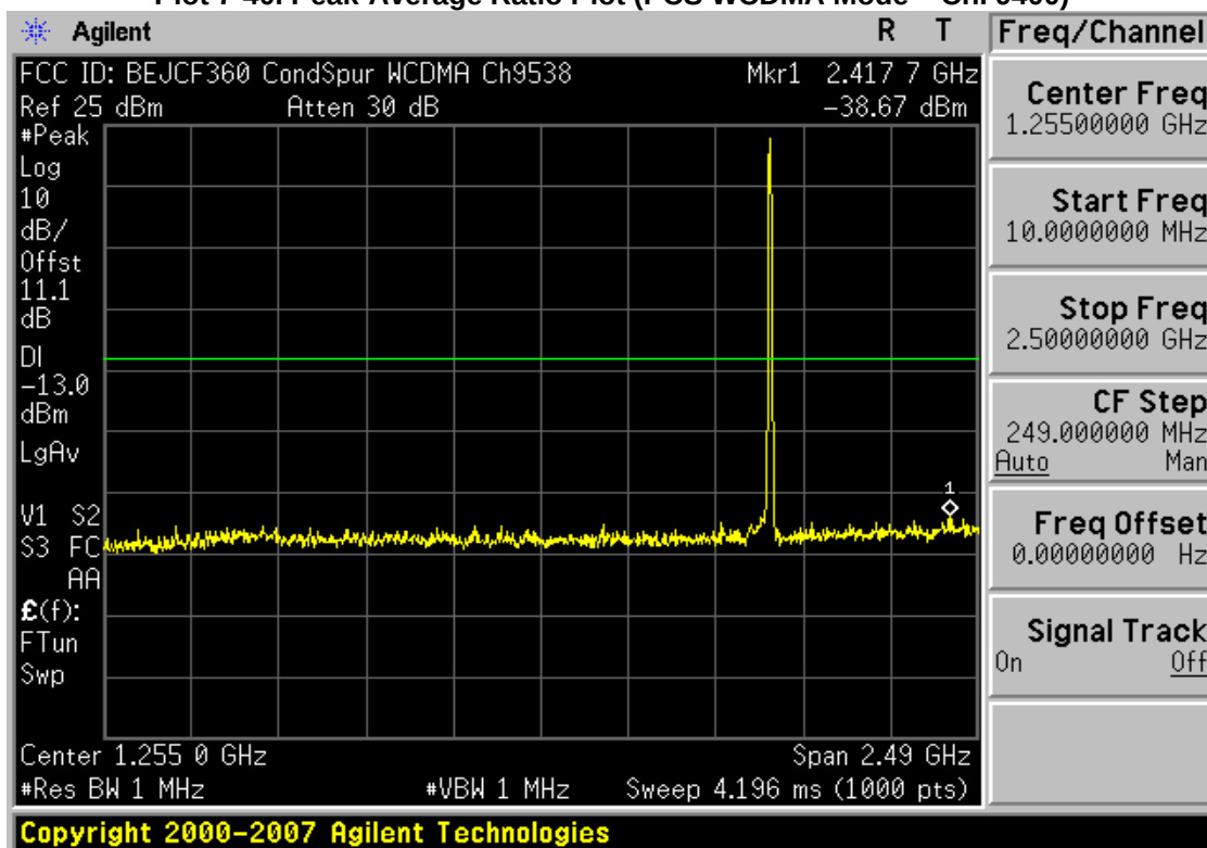
Plot 7-41. Conducted Spurious Plot (PCS WCDMA Mode - Ch. 9538)
