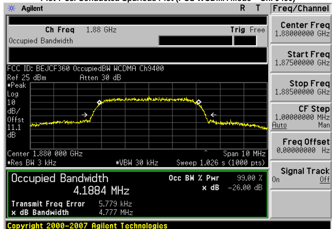
Plot 7-39. Occupied Bandwidth Plot (PCS WCDMA Mode – Ch. 9400)
