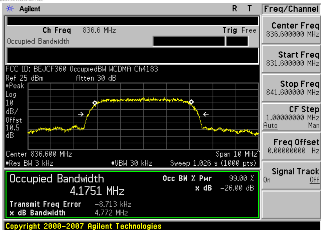
Plot 7-28. Occupied Bandwidth Plot (Cellular WCDMA Mode - Ch. 4183)
