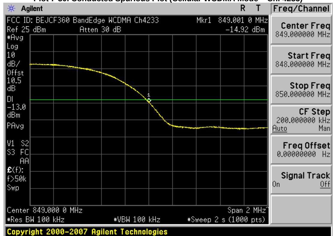
Plot 7-31. Band Edge Plot (Cellular WCDMA Mode – Ch. 4233)
