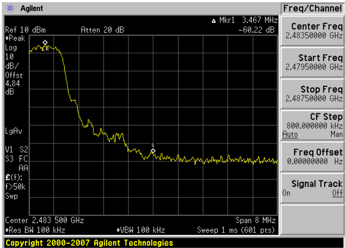
Plot 6-13. Band Edge Plot (Bluetooth, 2Mbps – Ch. 78)
