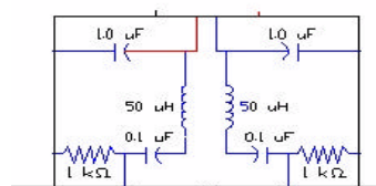
Figure 3-4. LISN Schematic Diagram
