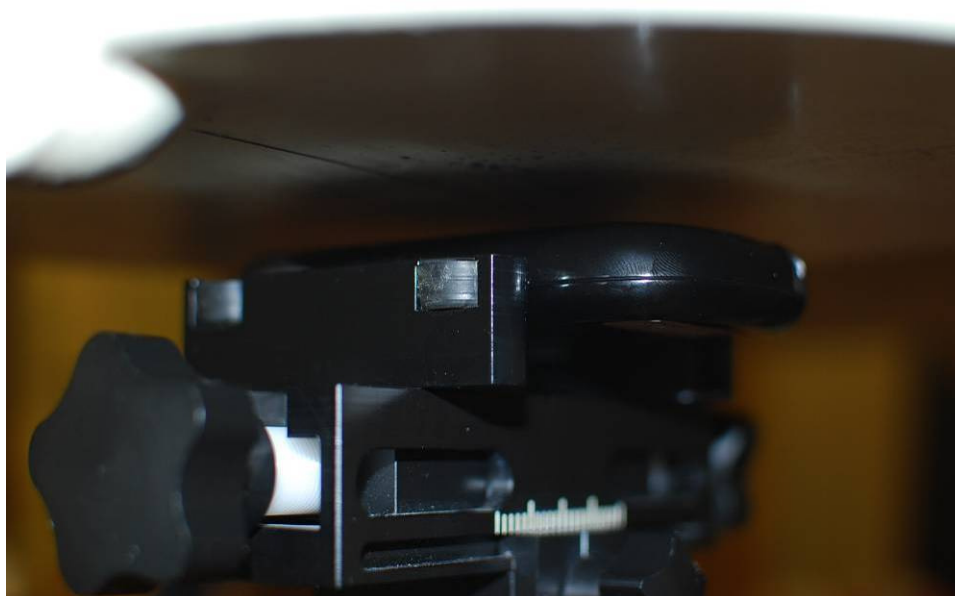
Figure 21-5 SAR Test Setup Photo 5 – Body Back
