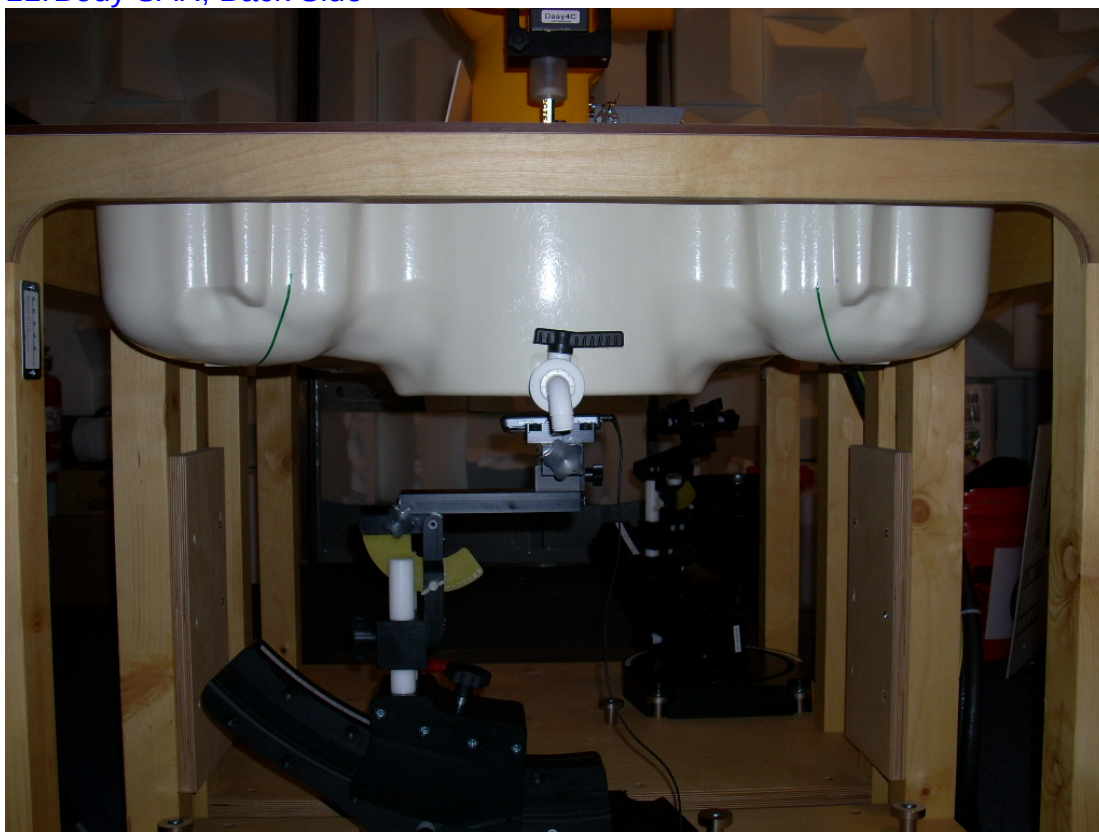
12. Body SAR, Back Side with 20mm Space
