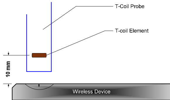
Figure 5-11 Measurement Distance
