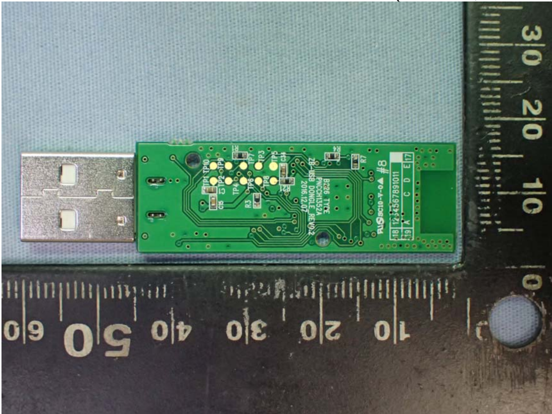
Figure 6 Internal View (I/O Board, Back View)
