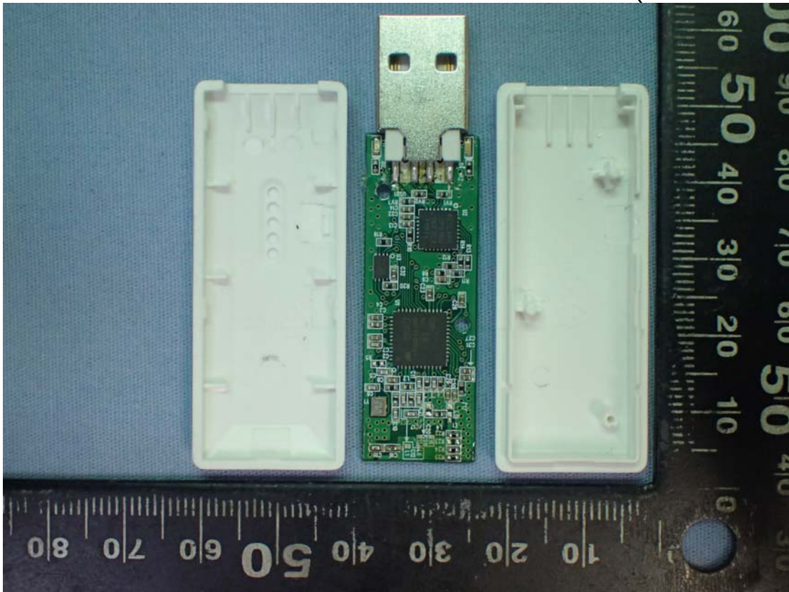
Figure 4 Internal View (RF IC)
