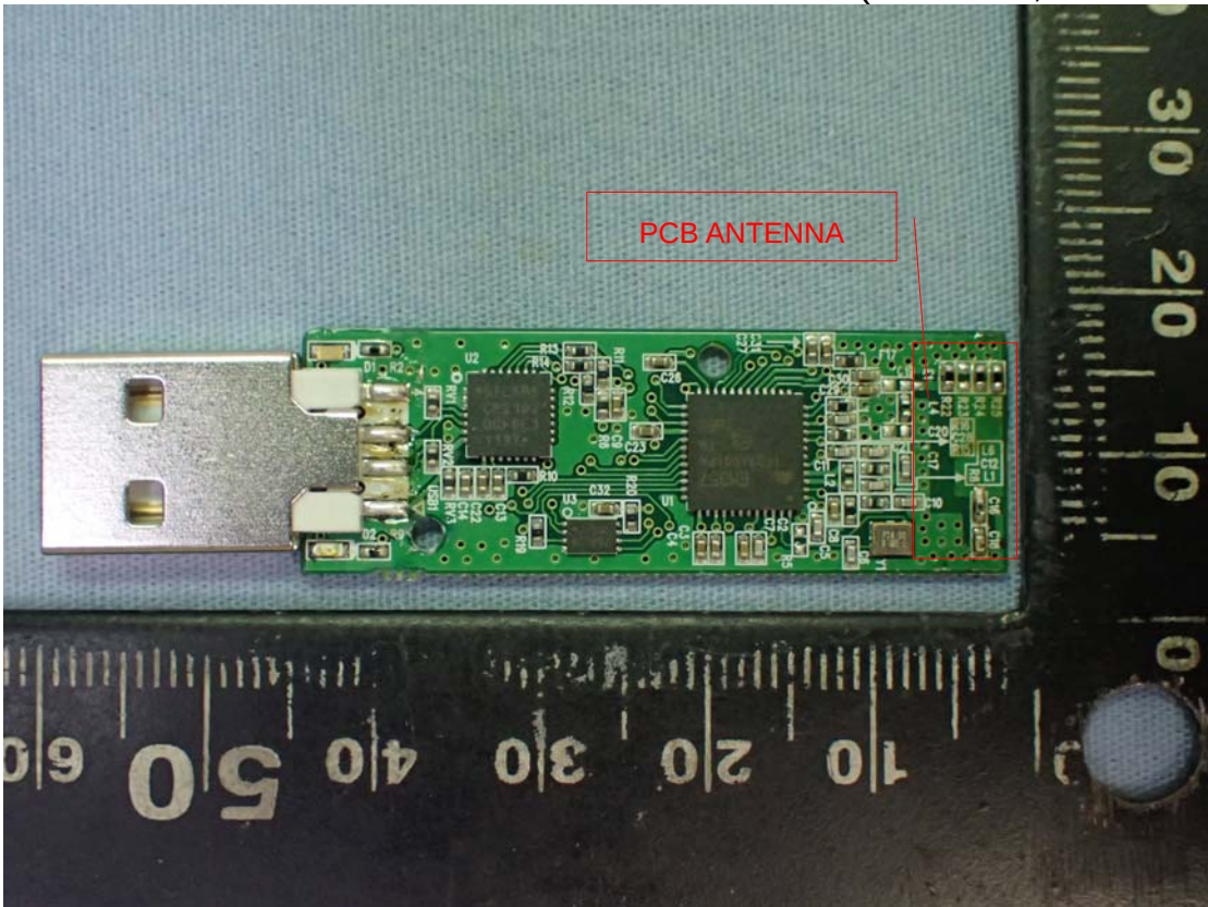
Figure 5 Internal View (I/O Board, Front View)
