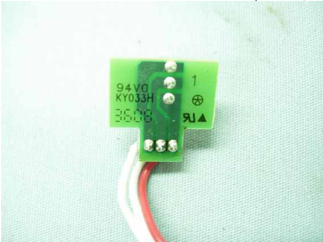
Figure 17 Internal View (LED Board, Front View)
