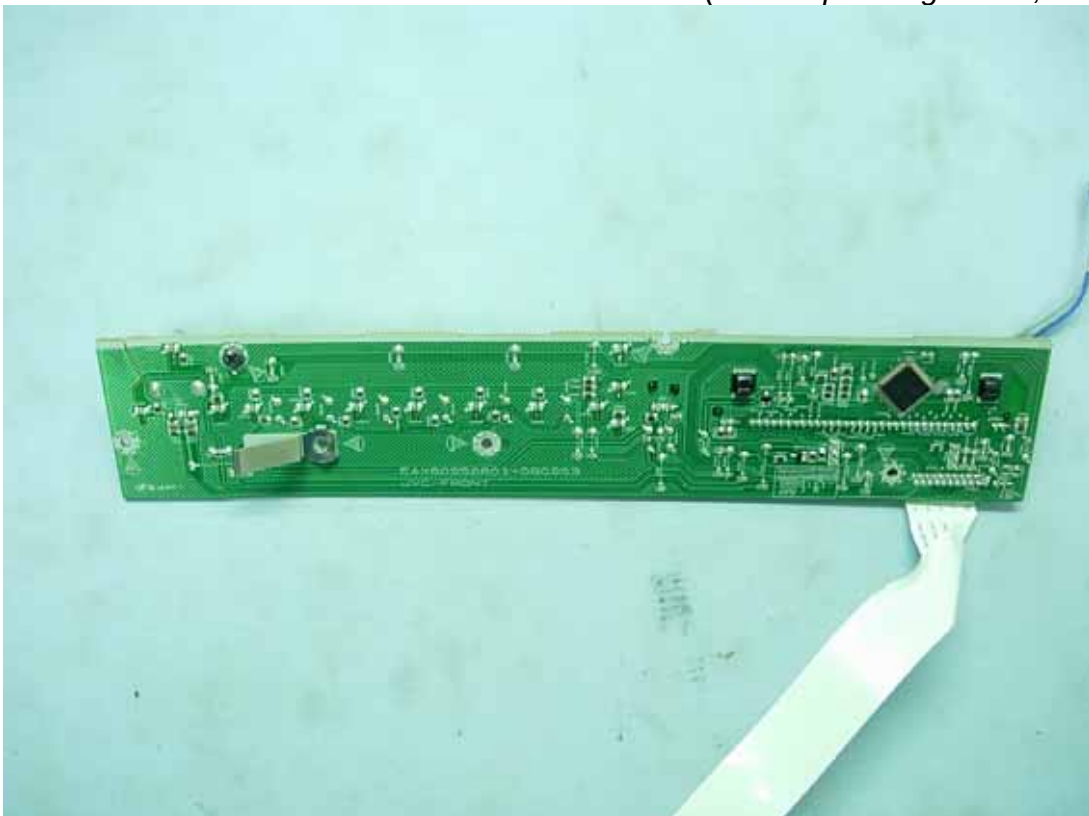
Figure 7 Internal View (Front Operating Board, Back View)
