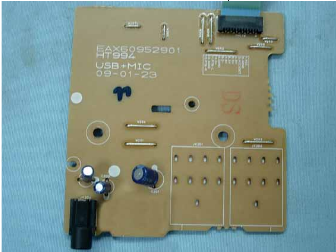
Figure 10 Internal View (Front Internal Board, Front View)
