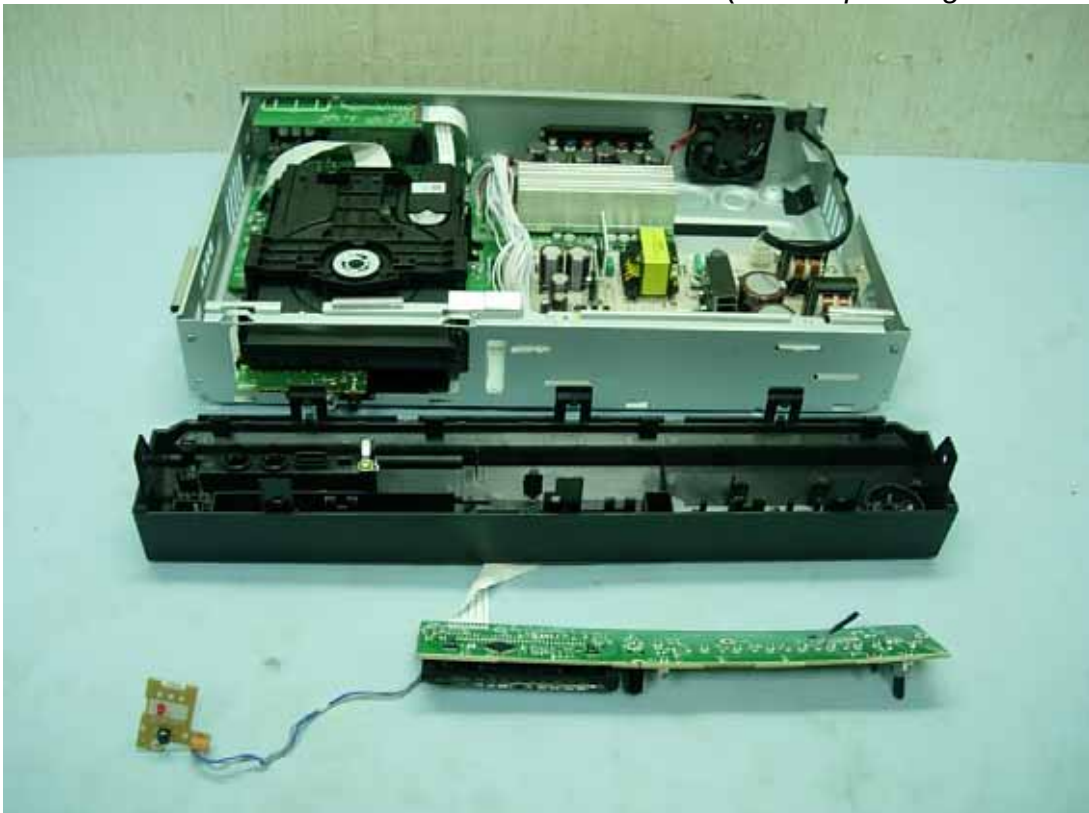
Figure 5 Internal View (Front Operating Board Removed)
