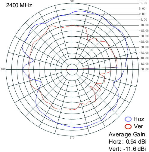
All Graphs in dBi
