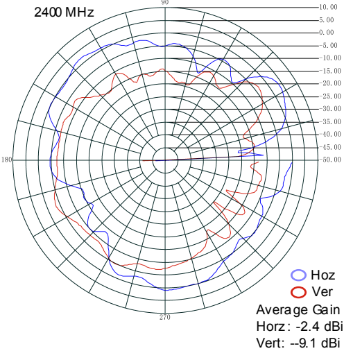
All Graphs in dBi
