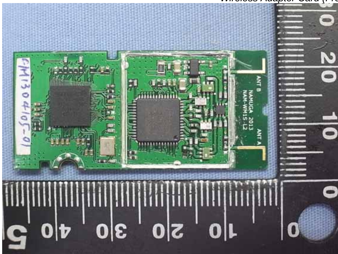
Wireless Adapter Card (Front View)
