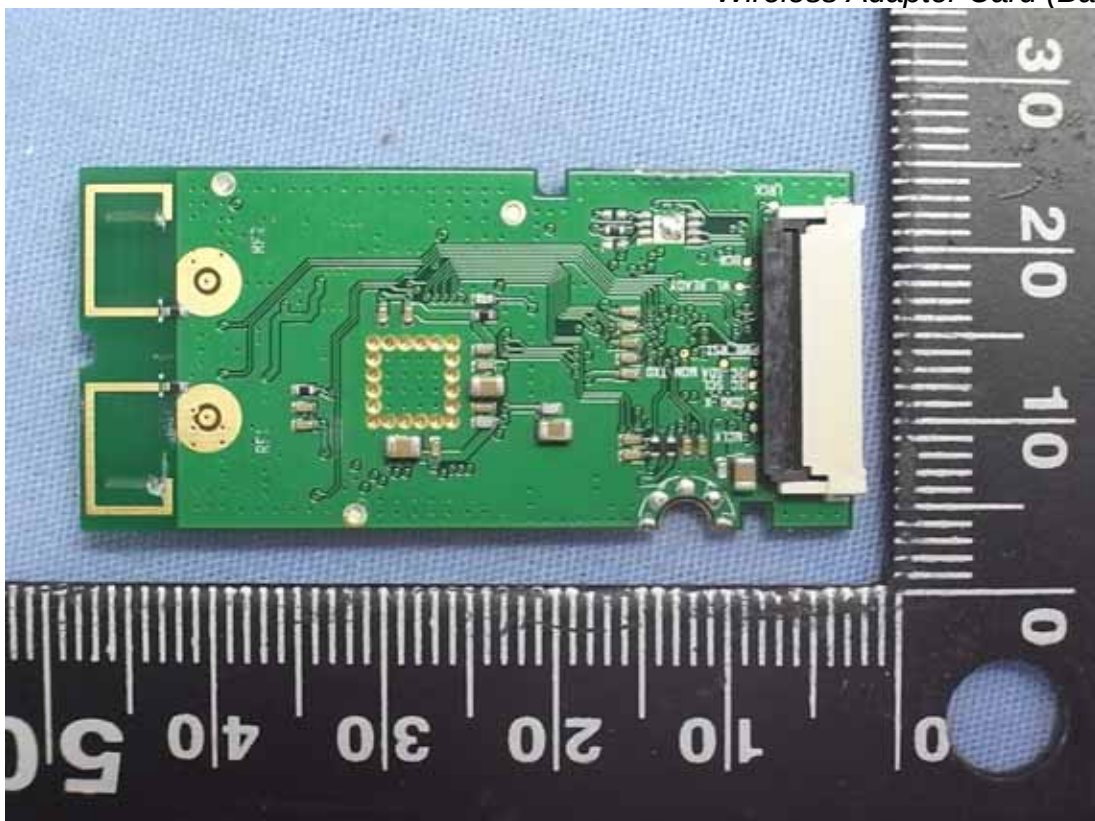
Figure 2 Wireless Adapter Card (Back View)
