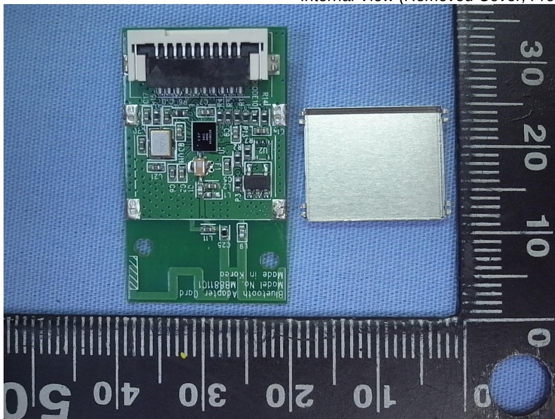
Figure 3 Internal View (Removed Cover, Front View)
