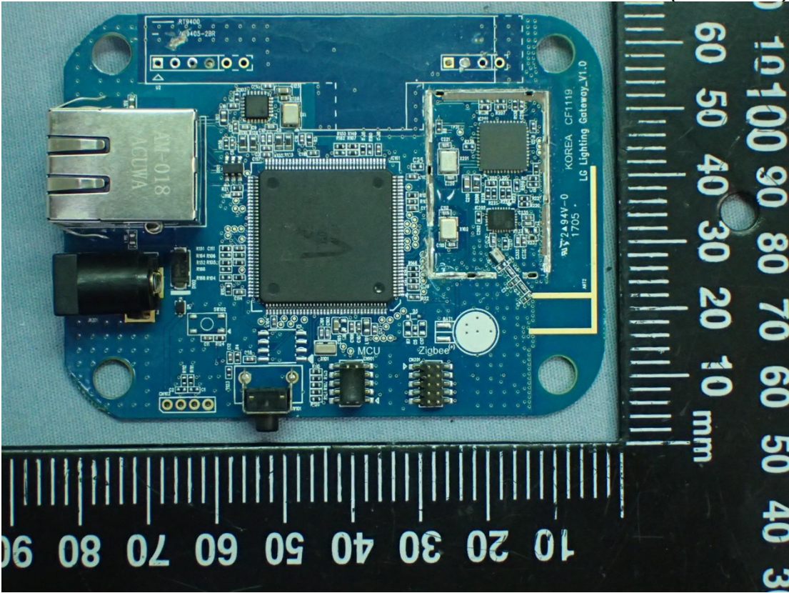
Figure 10 Main Board (Back View)
