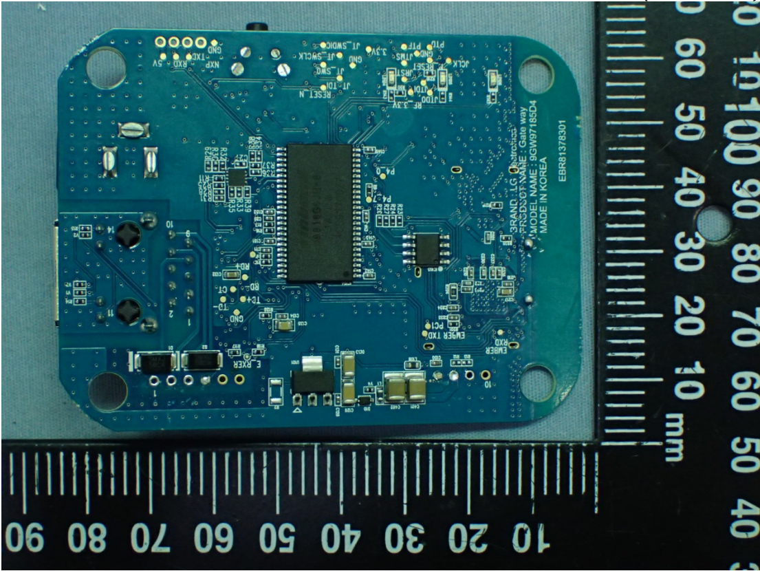
Figure 9 Main Board (Front View)
