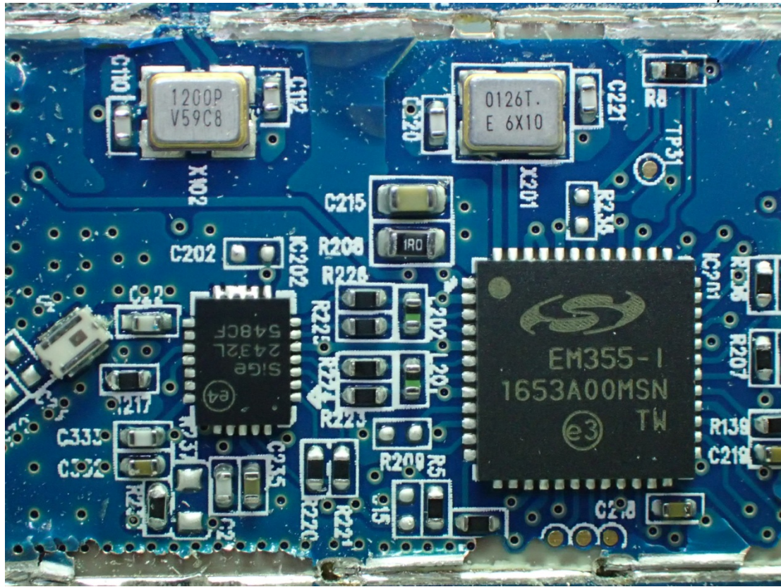
Figure 11 RF Chip View
