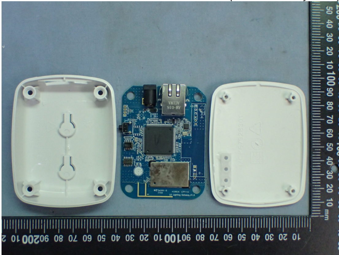
Figure 7 Internal View (Removed Battery Cover)
