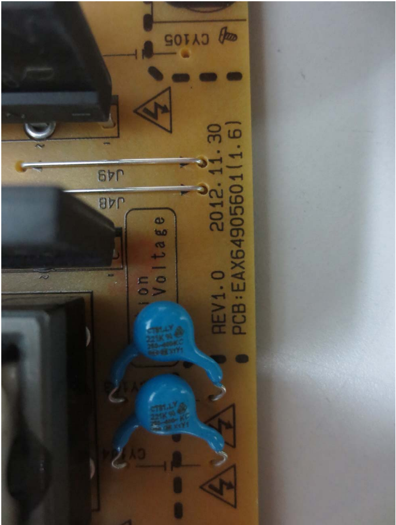
< Power Board Label2 >
