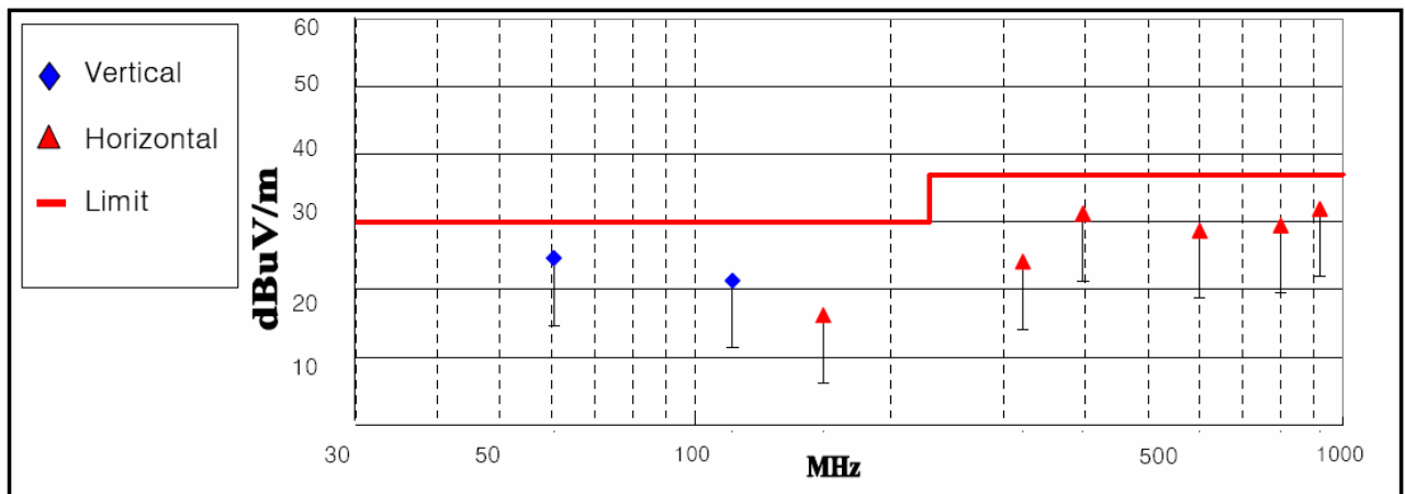
&lt; Fig 4. Radiated emission result _ Digital &gt;
