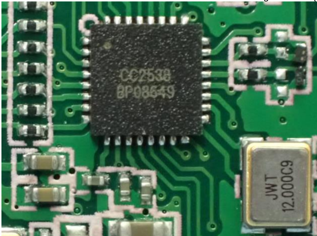
Figure 5 Original MCU (CC2538)
