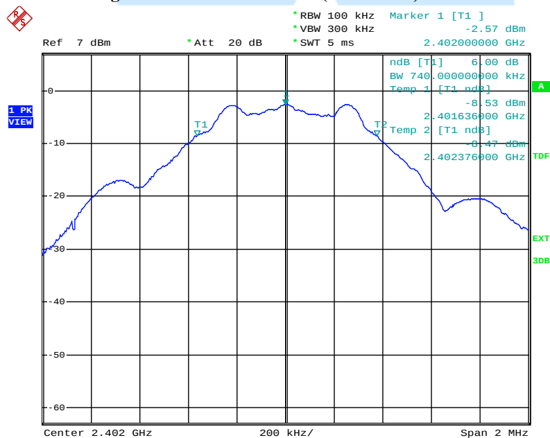
6 dB Bandwidth Plot on Configuration : Lowest channel (2 402 MHz)
