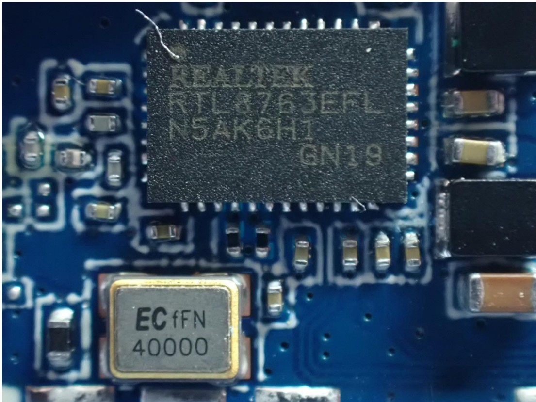
Figure 4 RF IC & Oscillator View
