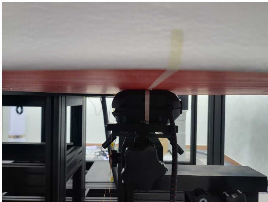
SAR Test Picture(Back), Test separation distance : 0 mm
