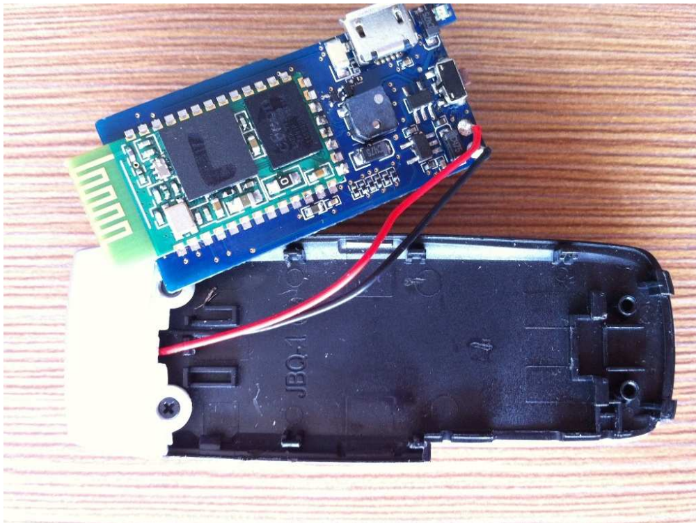
PCB rear side
