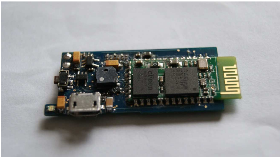
PCB rear side-detail
