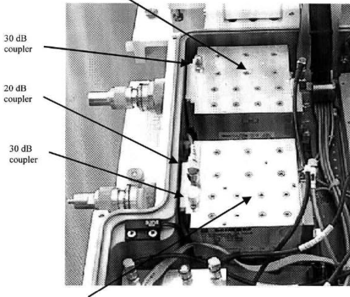
figure 2-5 Top view of the duplexers
