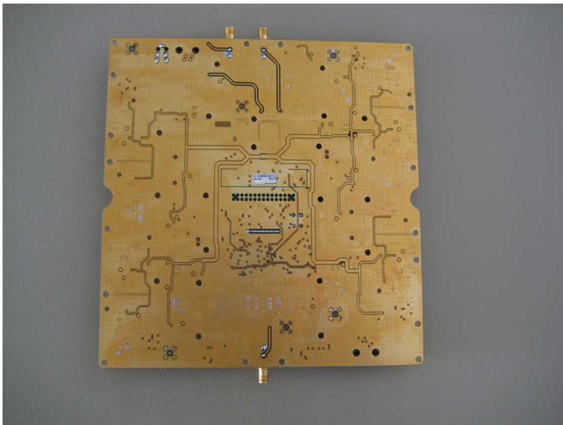
PCB back
