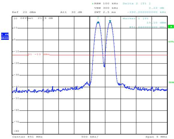
Figure 8.2-9: 5 MHz Intermodulation
