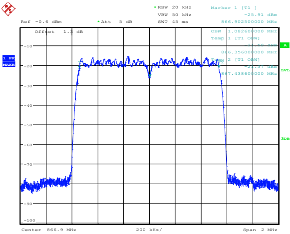
Figure 8.5-1: 1.4 MHz OFDM output
