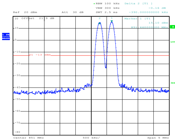
Figure 8.2-10: CDMA Intermodulation
