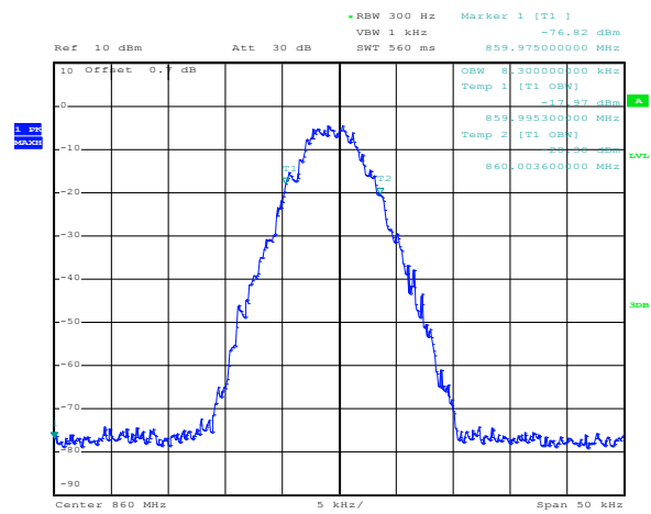
Figure 8.5-10: P25 output
