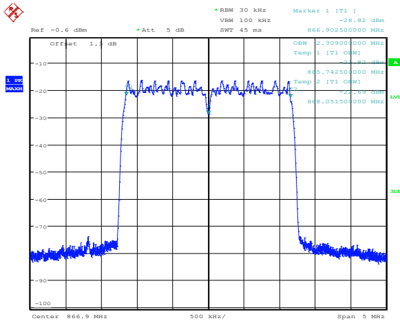
Figure 8.5-2: 3 MHz OFDM output
