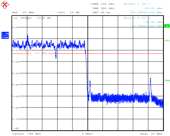
Figure 8.2-13: 5 MHz Intermodulation
