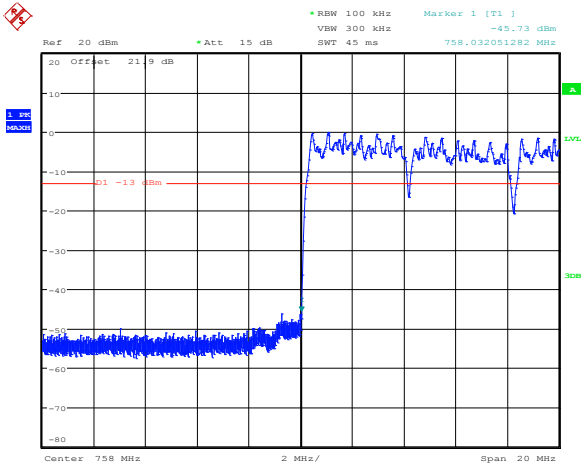
Figure 8.2-14: 5 MHz Intermodulation
