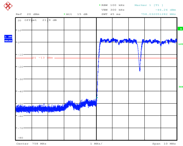
Figure 8.2-10: 1.4 MHz Intermodulation
