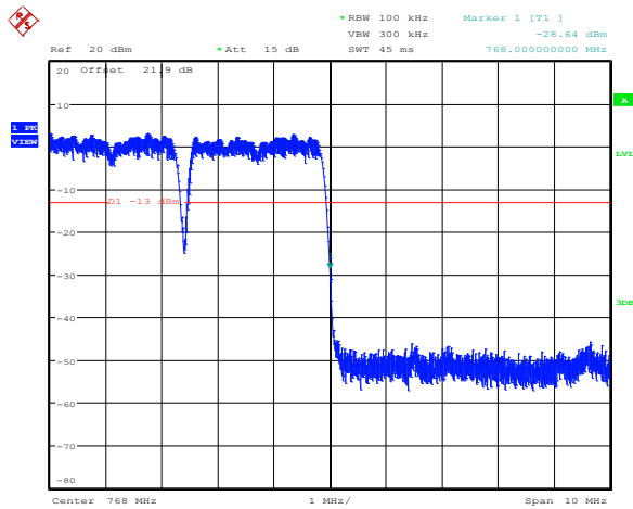
Figure 8.2-9: 1.4 MHz Intermodulation
