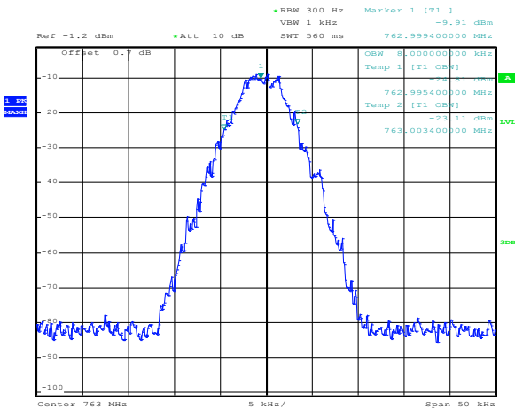
Figure 8.5-10: P25 output
