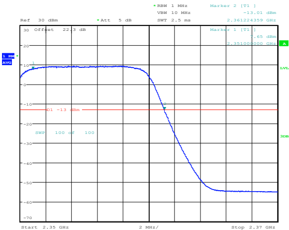
Figure 8.2-11: 10 MHz LTE QAM 2350 MHz
