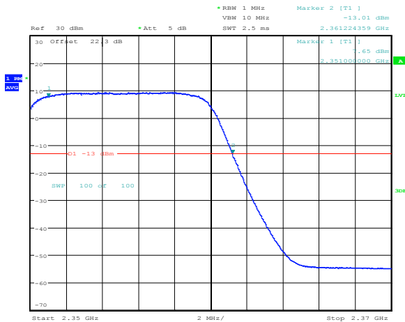
Figure 8.2-12: 10 MHz LTE QPSK 2350 MHz
