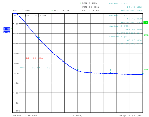
Figure 8.2-16: 10 MHz LTE QPSK 2360 MHz
