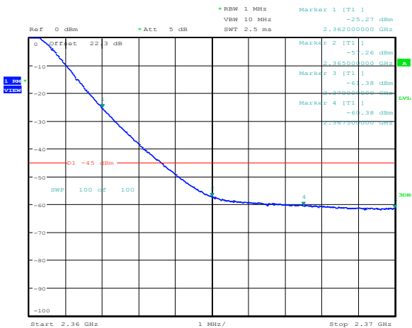
Figure 8.2-15: 10 MHz LTE QAM 2360 MHz
