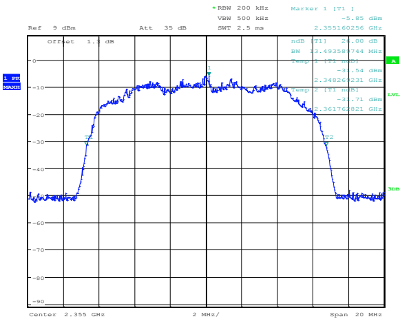
Figure 8.5-1: 10 MHz QAM output
