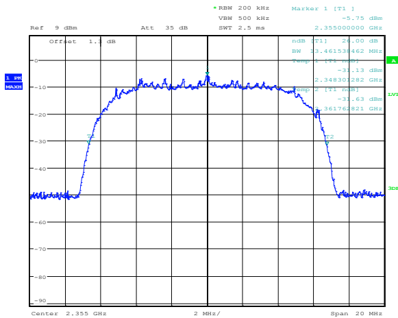
Figure 8.5-2: 10 MHz QPSK output
