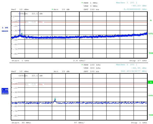
Figure 8.2-6: 15 MHz LTE QPSK 30 MHz 27 GHz
