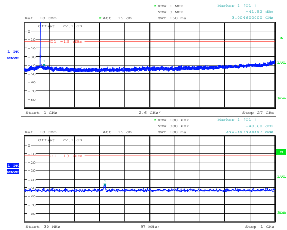
Figure 8.2-2: 5 MHz LTE QPSK 30 MHz 27 GHz
