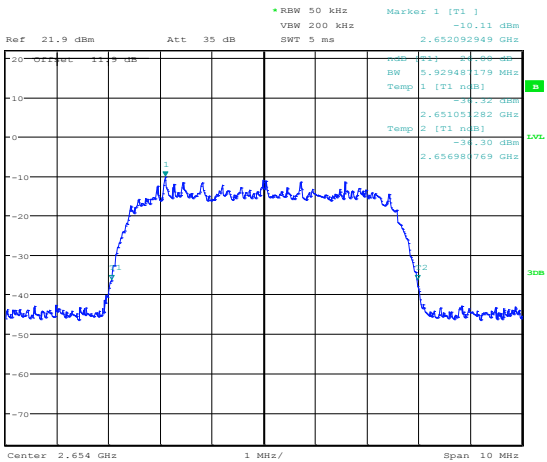
Figure 8.5-2: 5 MHz QPSK output
