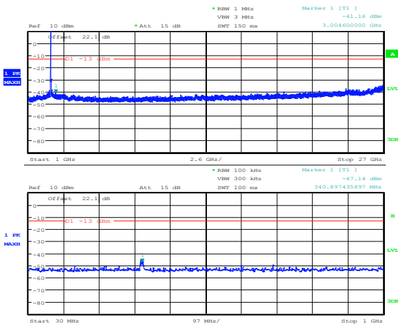
Figure 8.2-1: 5 MHz LTE QAM 30 MHz 27 GHz
