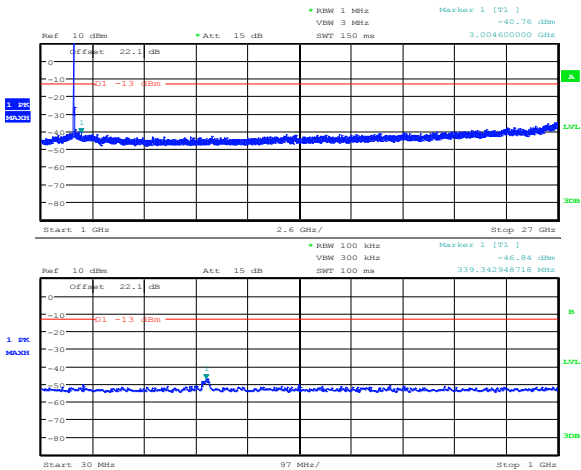
Figure 8.2-5: 15 MHz LTE QAM 30 MHz 27 GHz
