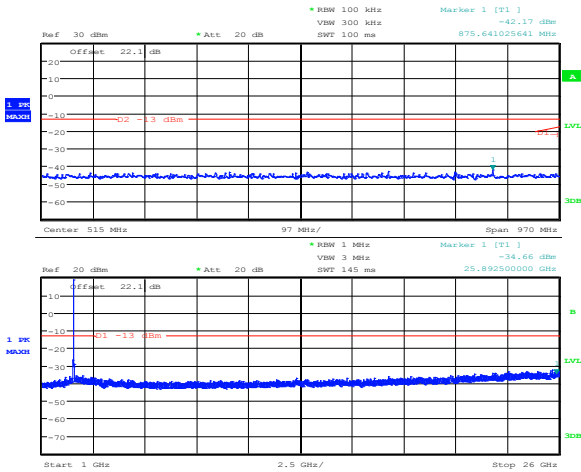
Figure 8.2-2: 5 MHz LTE QPSK 30 MHz 26 GHz
