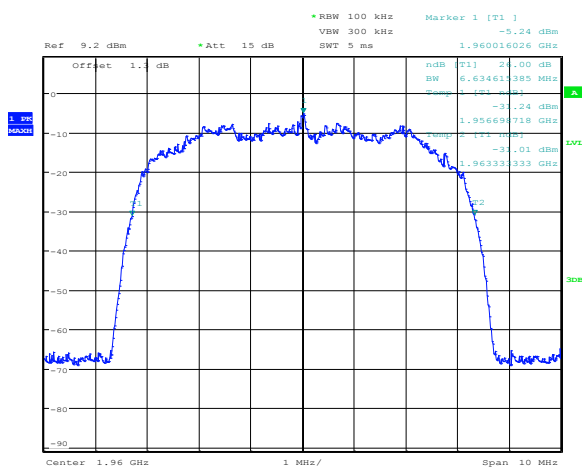
Figure 8.5-9: 5 MHz QAM output
