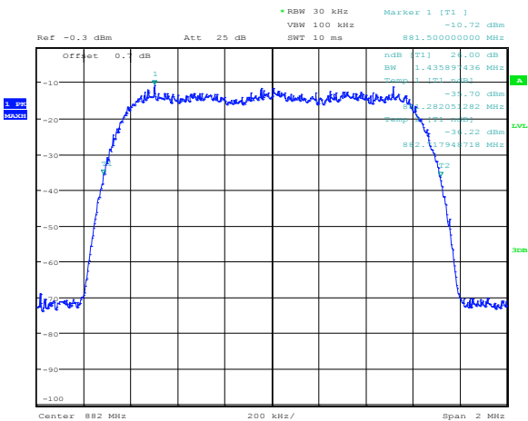
Figure 8.5-17: CDMA output
