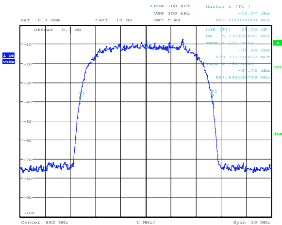
Figure 8.5-18: 10 UMTS output
