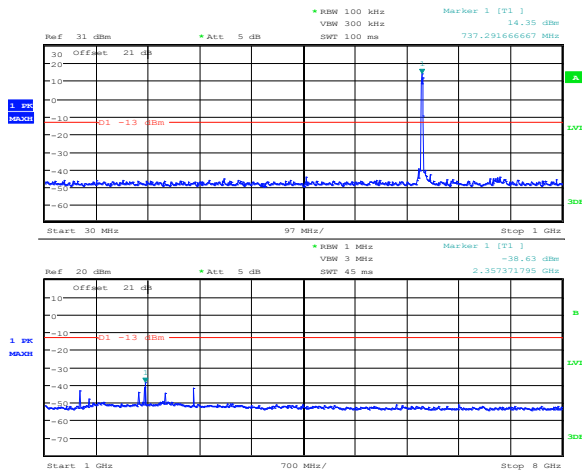
Figure 8.2-2: 1.4 MHz LTE QPSK 30 MHz – 8 GHz
