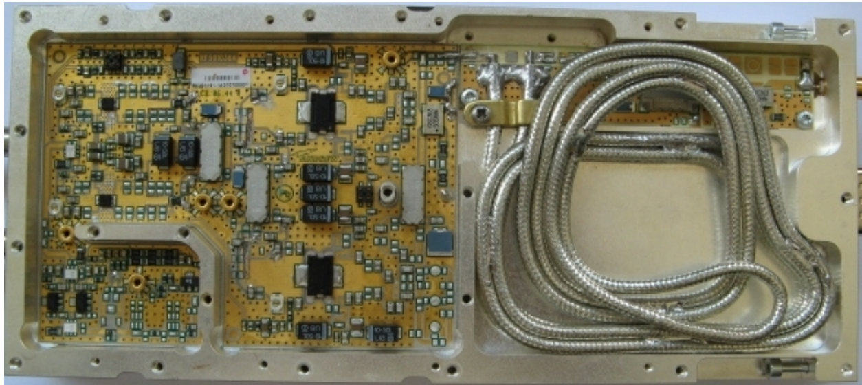
PA 800 MHz - Bottom
