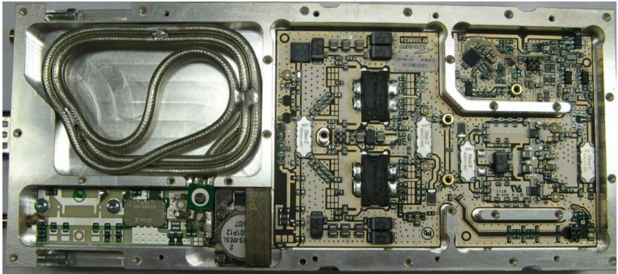
PA 1900 MHz - Bottom
