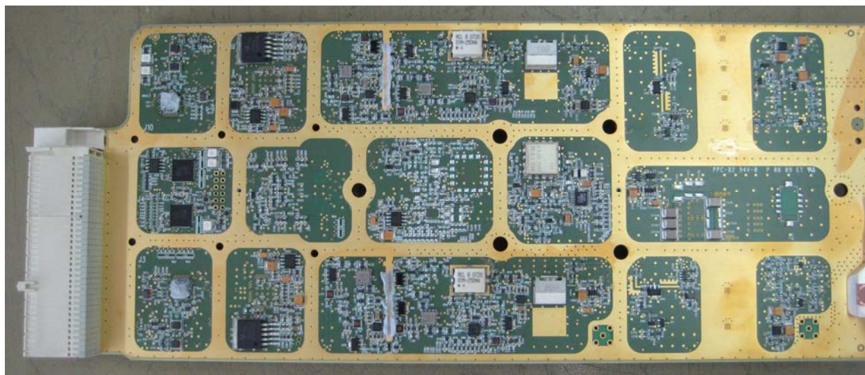
RF Board Bottom
