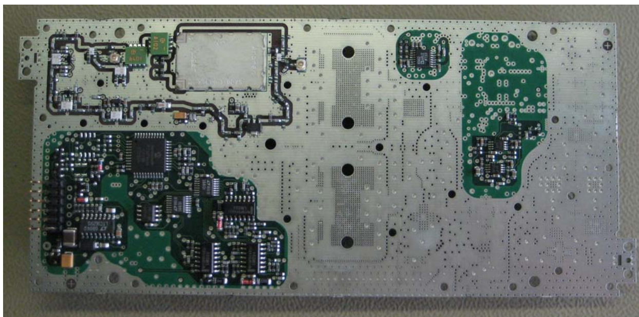
Final PA Board Bottom
