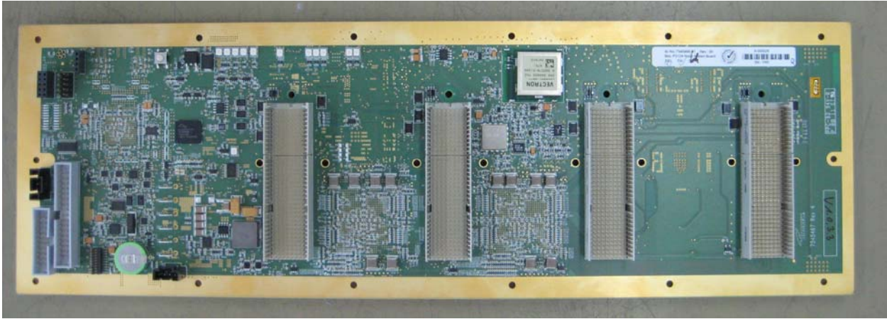
Main Board Top
