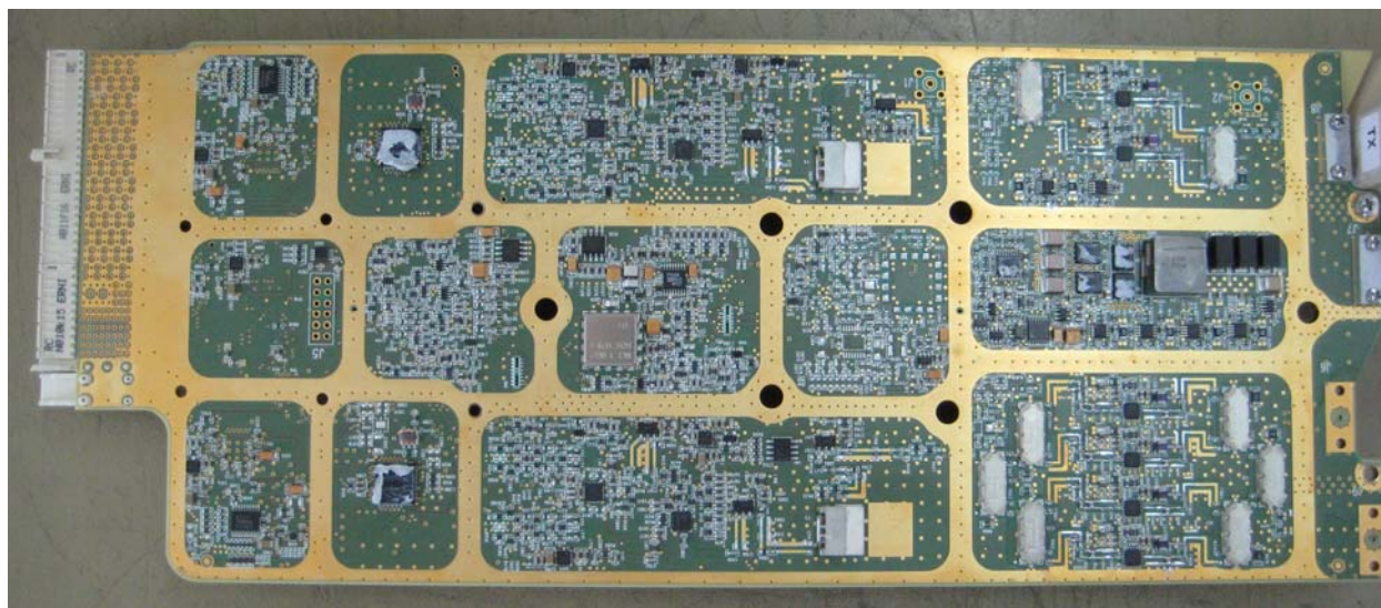
RF Board Top
