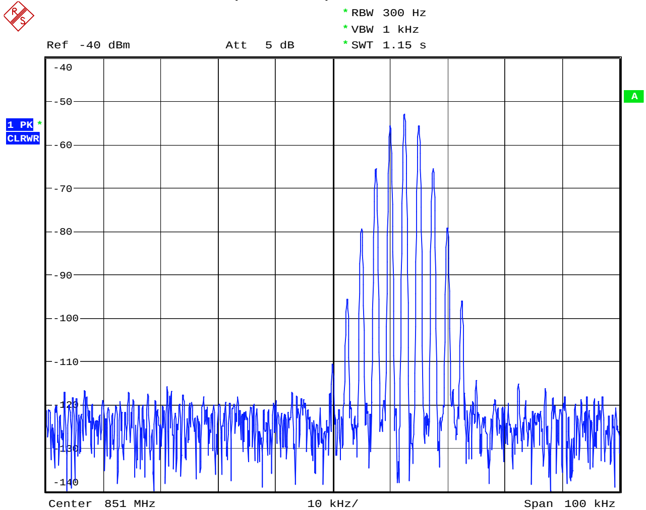
Figure 13 Analogue Input Downlink – FM 2.5 kHz tone @ 3 kHz deviation – Low Channel (851.0125 MHz)
