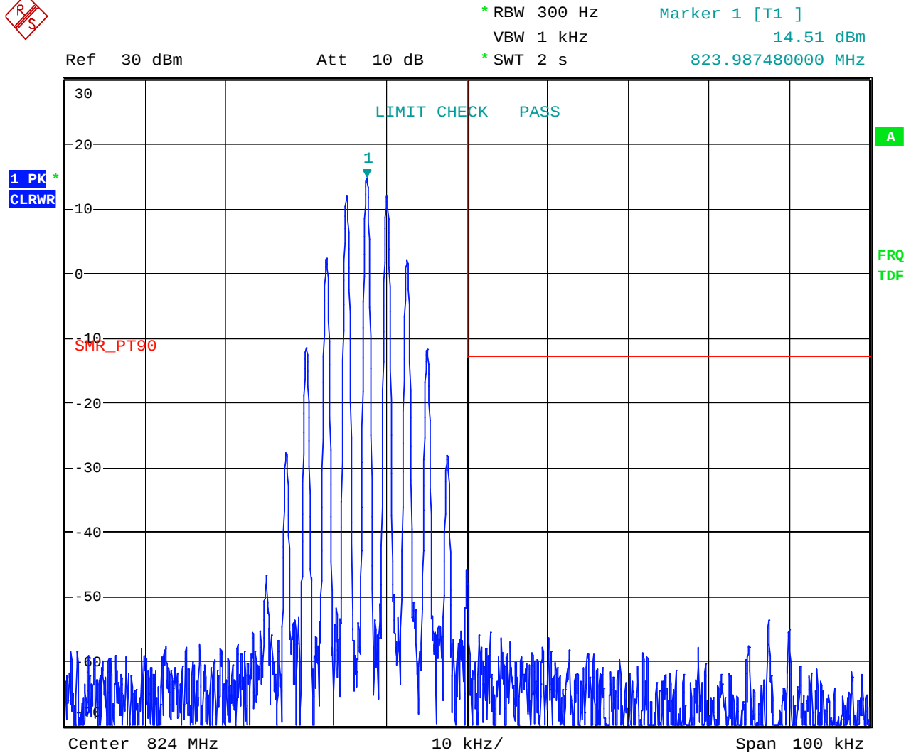
Figure 6 Analogue Output Uplink - FM 2.5 kHz tone @ 3 kHz deviation – Upper Channel (823.9875 MHz)
