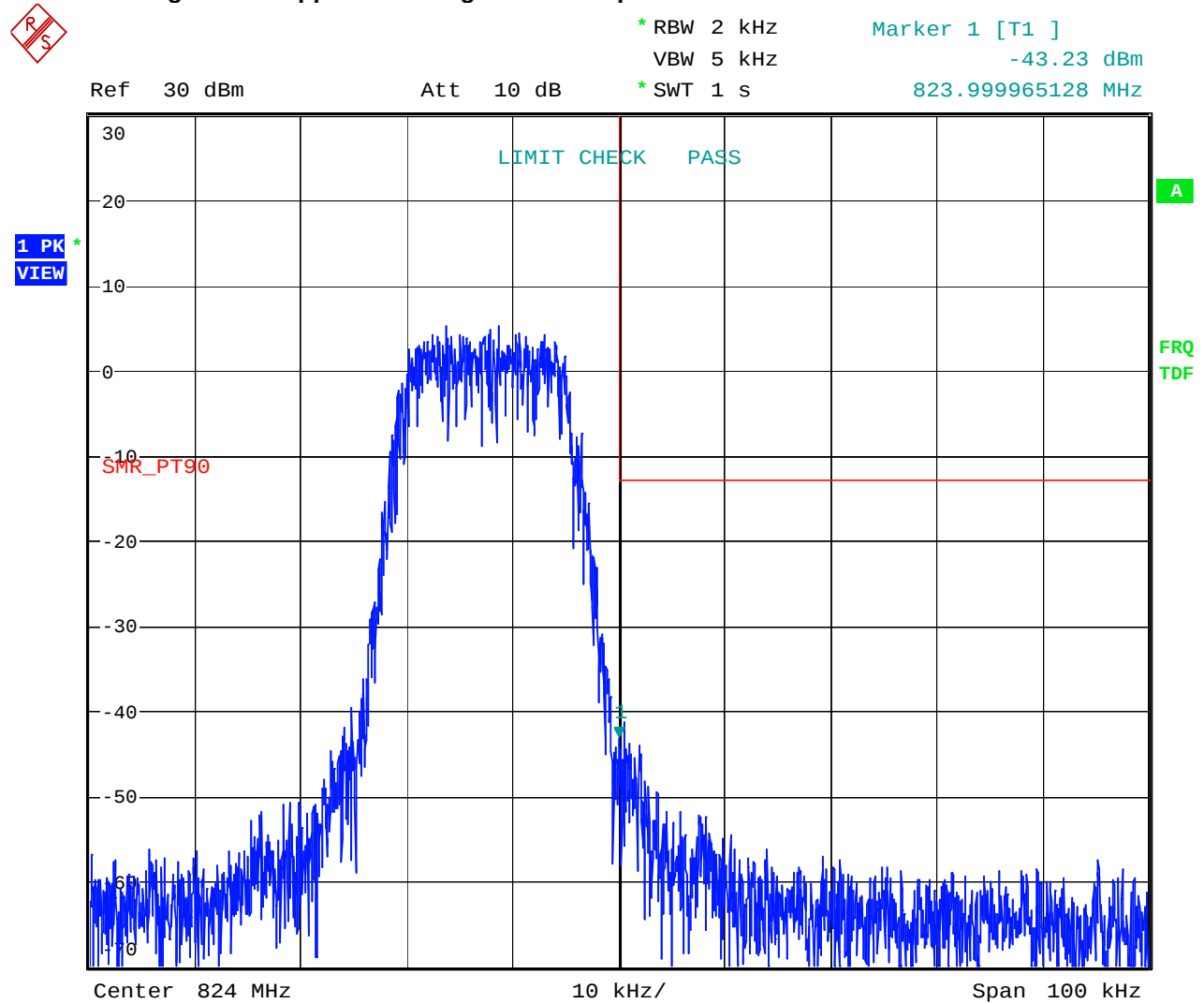
Figure 38 Upper Band Edge – iDEN - Uplink
