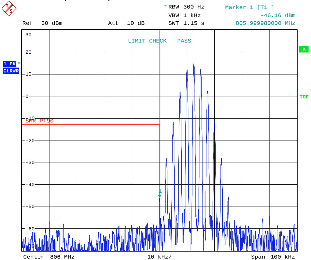
Figure 2 Analogue Output Uplink - FM 2.5 kHz tone @ 3 kHz deviation – Low Channel (806.0125 MHz)
