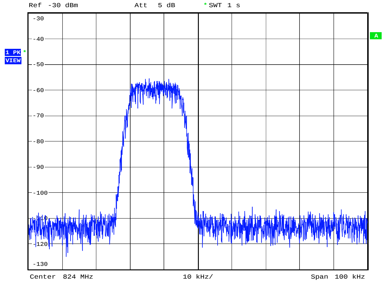
Figure 11 iDEN Waveform Input Uplink – Upper Channel (823.9875 MHz)
