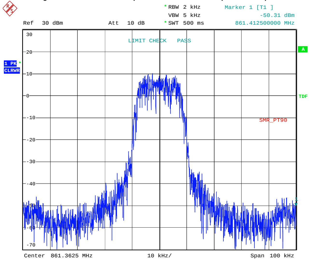
Figure 22 iDEN Waveform Output Downlink – Mid Channel (861.3625 MHz)
