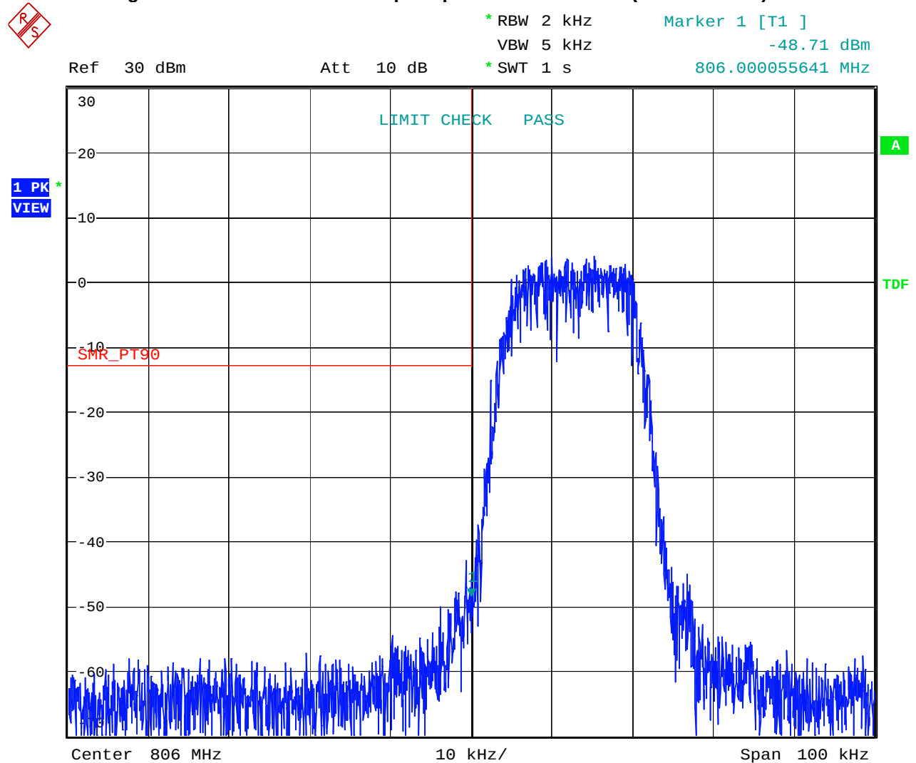
Figure 8 iDEN Waveform Output Uplink – Low Channel (806.0125 MHz)
