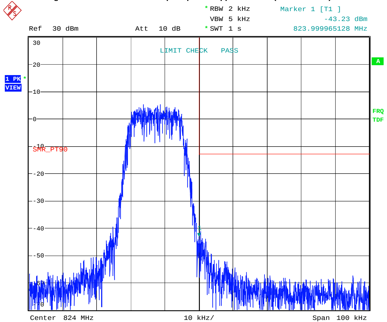
Figure 12 iDEN Waveform Output Uplink – Upper Channel (823.9875 MHz)
