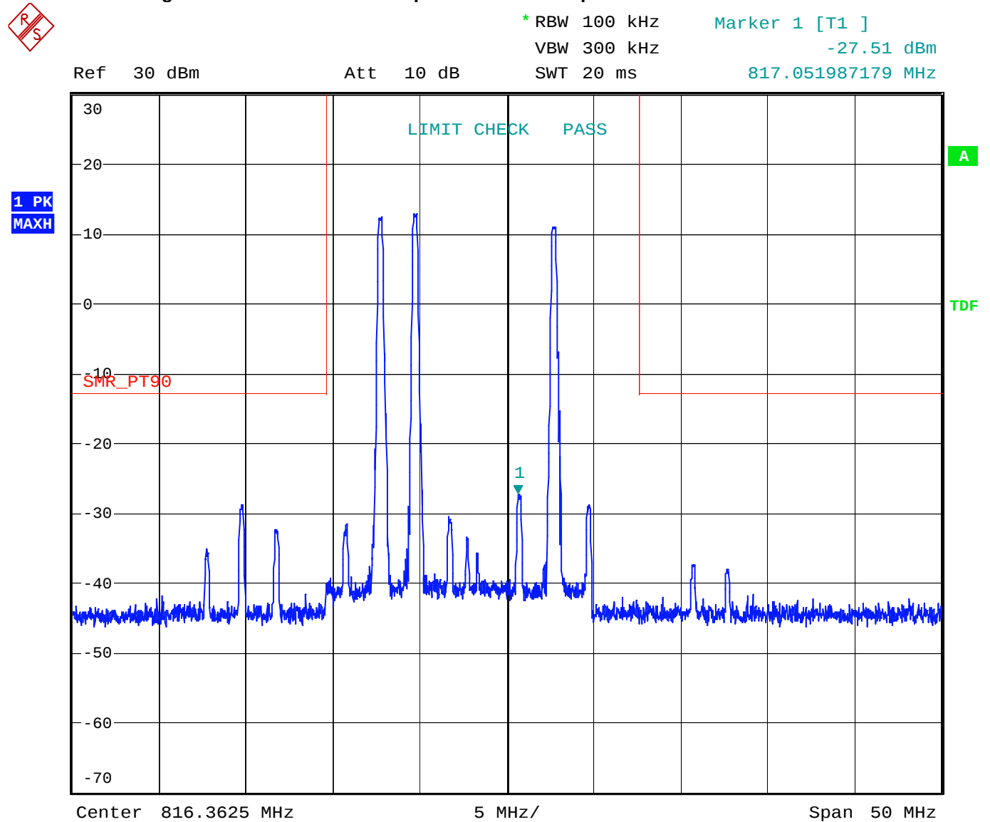
Figure 30 Intermodulation Spurious – iDEN - Uplink
