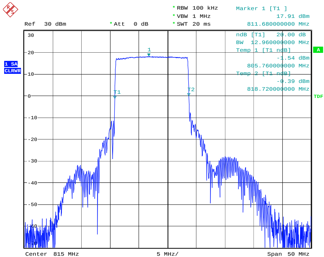
Figure 42 Uplink – 20 dB Bandwidth
