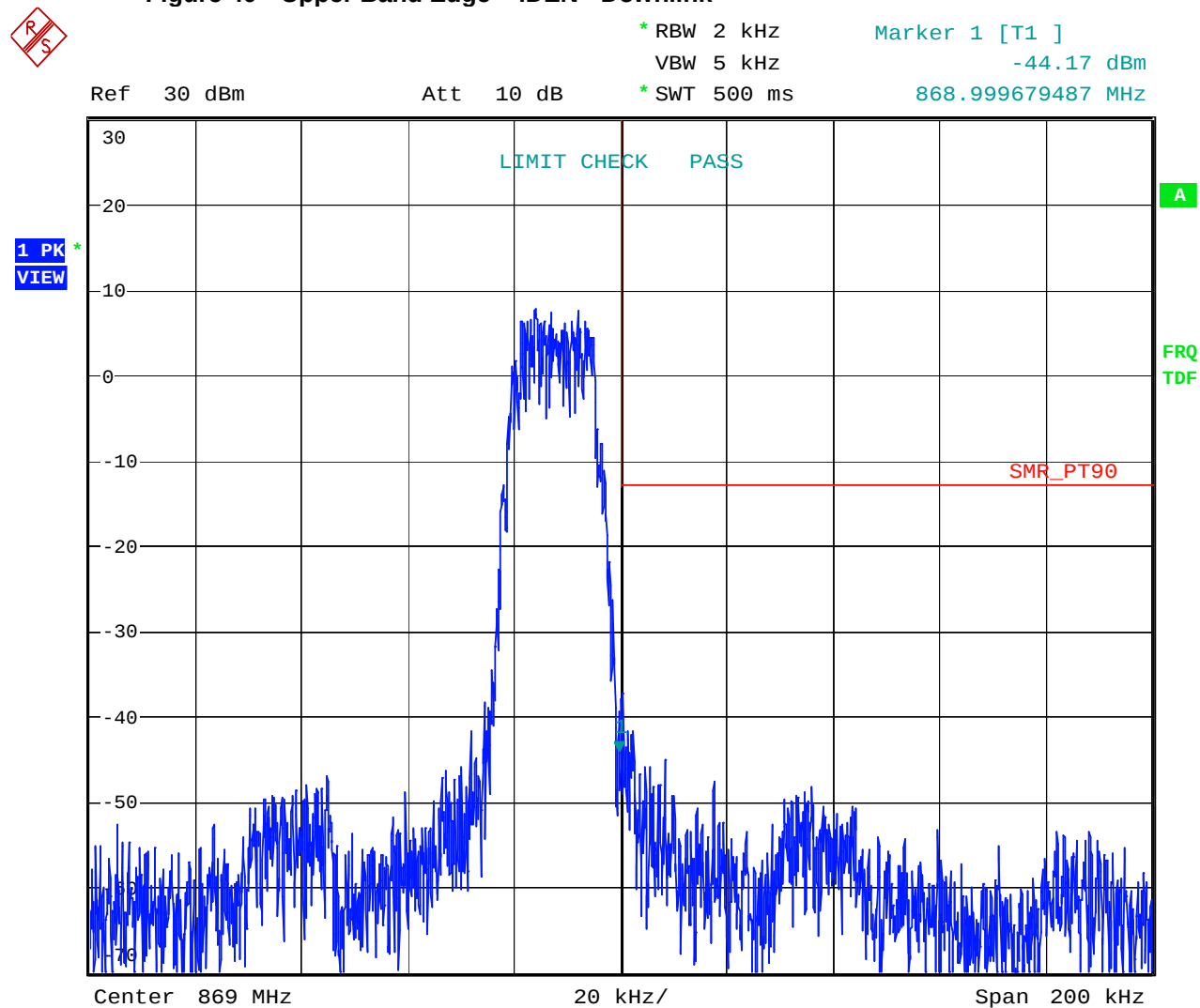
Figure 40 Upper Band Edge – iDEN - Downlink
