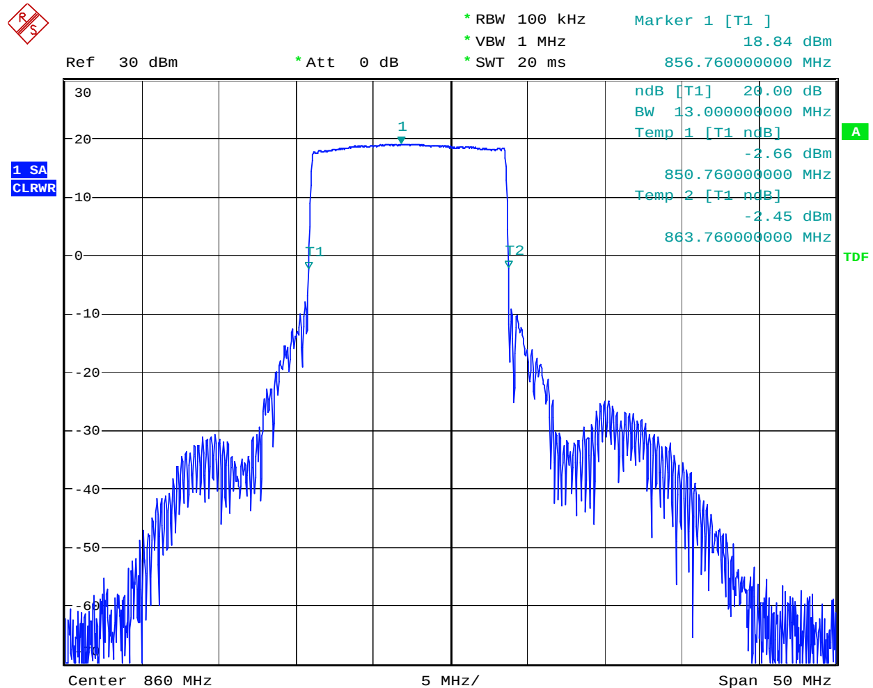
Figure 41 Downlink – 20 dB Bandwidth
