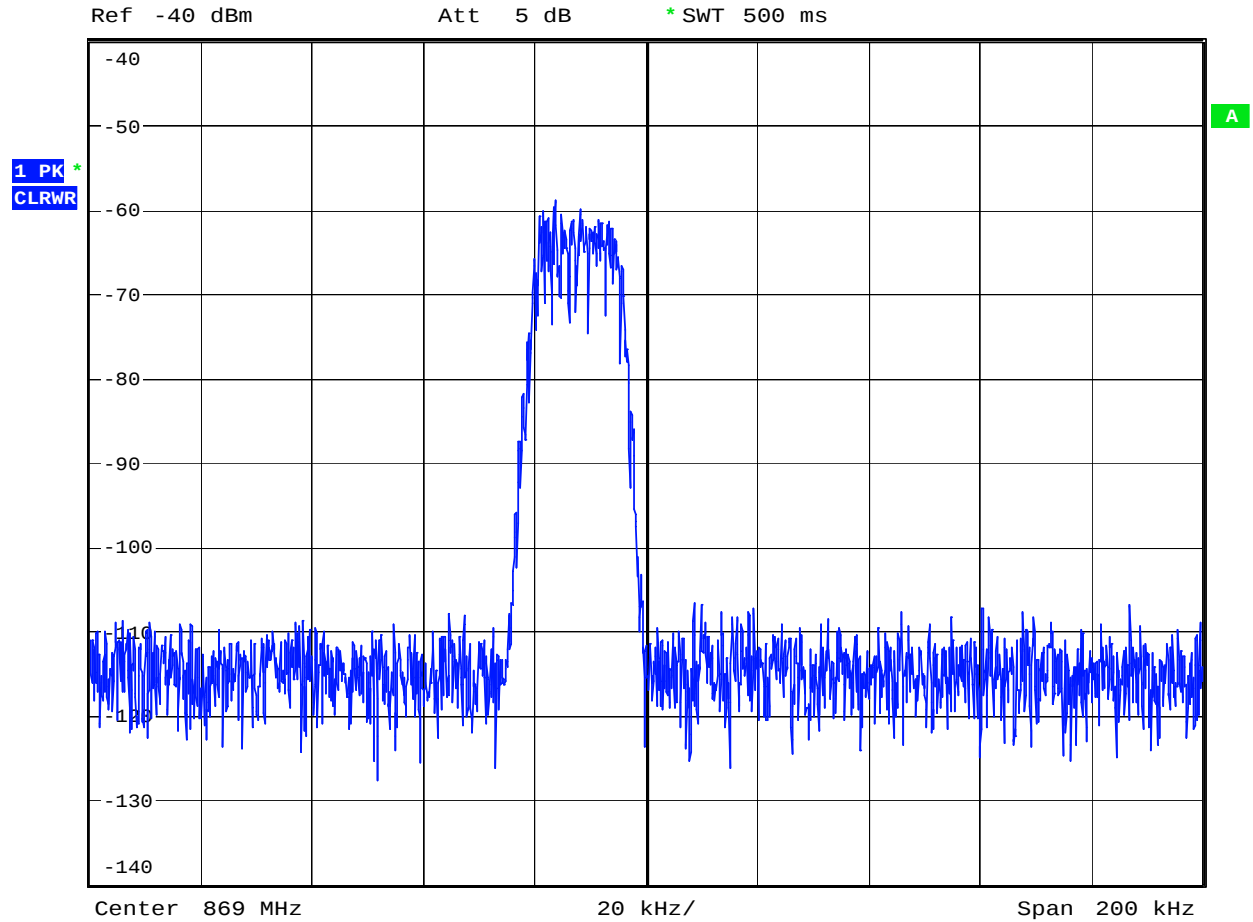
Figure 23 iDEN Waveform Input Downlink – Upper Channel (868.9875 MHz)
