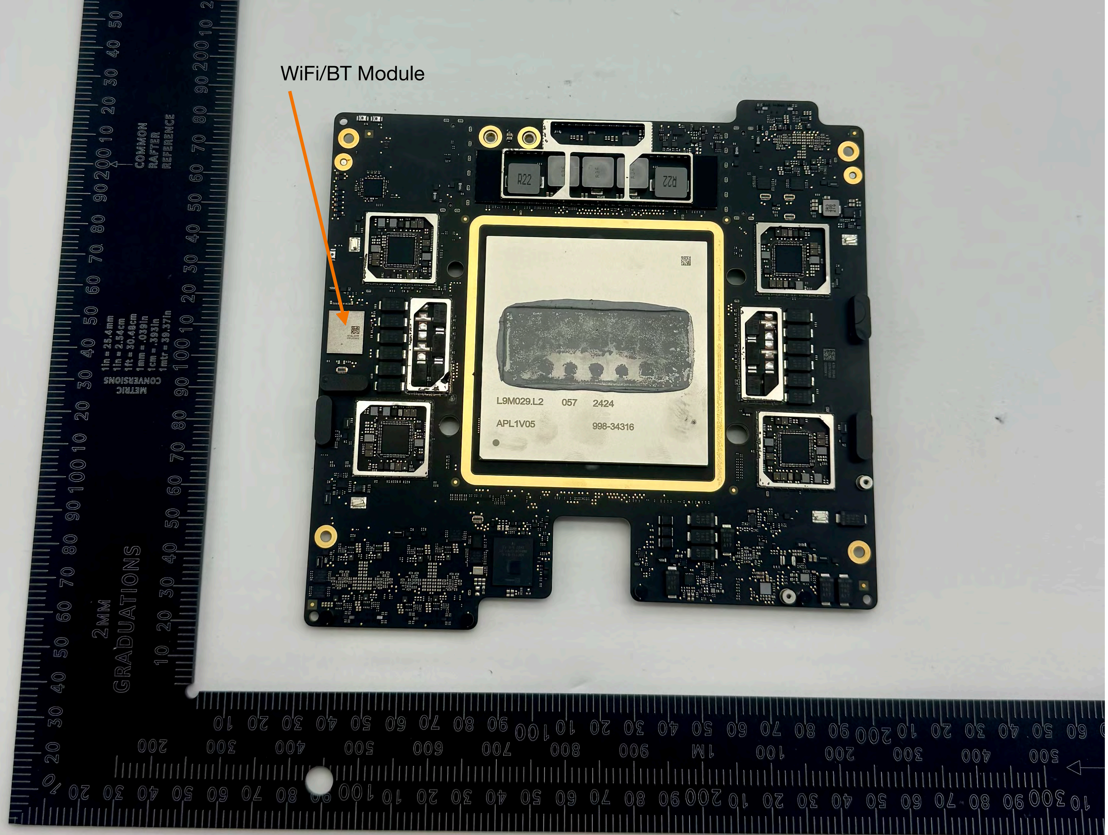
A3389 MLB with shield removed - Top
